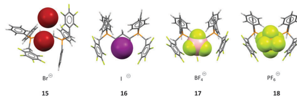
Fig. 8 View of the ion pairs of the 1,3-bis(diphenylpentafluorobenzylphosphonium) propane salts 15 – 18 as observed in the solid state showing the individual or simultaneous interaction of the C 6 F 5 units with the anion. 24b
