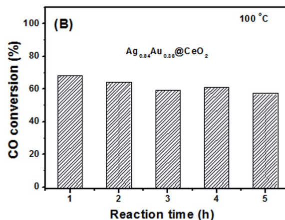
Fig. 4 (A) CO conversion curves of \text{Ag}@CeO_2 , \text{Ag}_{0.64}\text{Au}_{0.36}@CeO_2 , \text{Ag}_{0.41}\text{Au}_{0.59}@CeO_2 and \text{Au}@CeO_2 ; (B) cycling test of \text{Ag}_{0.64}\text{Au}_{0.36}@CeO_2 at 100 \text{ }^\circ\text{C} for 5 h.
