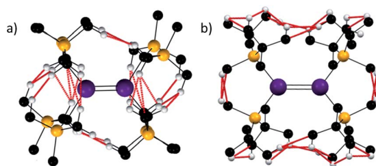
Fig. 3 H–H and C–H distances below the sum of the van der Waals radii (2.4 and 2.9 Å respectively indicated in red) for [Sn{CH(SiMe 3 ) 2 } 2 ] 2 (a) and [Sn{SiMe 2 Bu 2 } 2 ] 2 (b).
