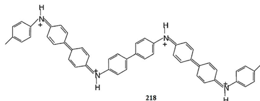
Fig. 182 Bipolaronic form of PDPA 218.
