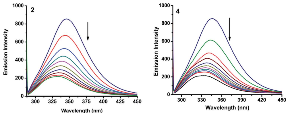
Fig. 11 Fluorescence quenching curves of BSA in the absence and presence of 2 and 4. [BSA] = 1 \mu M and [complex] = 0–50 \mu M.
