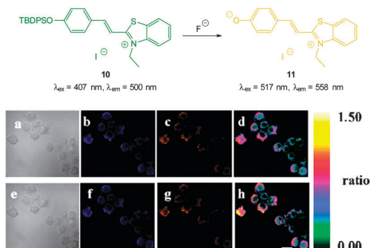
Fig. 9 Top: structure and reaction of benzothiazolium hemicyanine 10 with \text{F}^- . Bottom: images of RAW264.7 macrophages incubated with 10 and no added \text{F}^- (a) bright-field, (b) blue channel at 490 \pm 20 \text{ nm} , (c) orange channel at 560 \pm 20 \text{ nm} , and (d) ratio image from (c) and (b). Images of RAW264.7 macrophages incubated with 6 after addition of NaF (e) bright-field, (f) blue channel at 490 \pm 20 \text{ nm} , (g) orange channel at 560 \pm 20 \text{ nm} , and (h) ratio image from (g) and (f). Scale = 20 \mu\text{m} . Image reproduced with permission. 122
