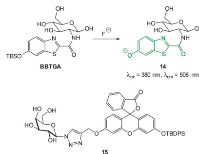
Fig. 12 Structure of BBTGA and 15 , showing reaction of BBTGA with \text{F}^- .
