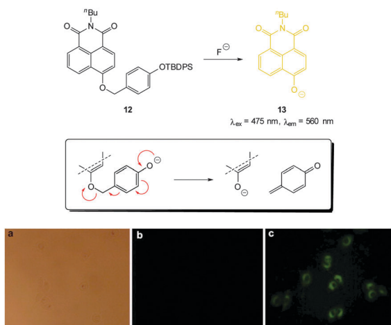
Fig. 10 Top: functionalised naphthalimide probe 12 and its reaction with \text{F}^- ; inset shows fragmentation mechanism. Bottom: (a) bright-field image of A549 cells incubated with 12 ( 20 \mu\text{M} ) for 24 h (a) bright field (b) without NaF (c) with NaF ( 50 \text{ mM} ). Image reproduced with permission. 123
