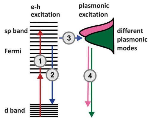
Fig. 5 A solid state model explanation of the plasmonic related 2PPL emission from nanostructures. Step 1: two-photon excitation from the d band to the sp band. Step 2: interband relaxation producing 2PPL photons. Step 3: energy transfer from the excited sp band to the plasmonic modes of slightly different energies. Step 4: radiative decays from the plasmonic modes to the d band giving rise to 2PPL of slightly different energies.
