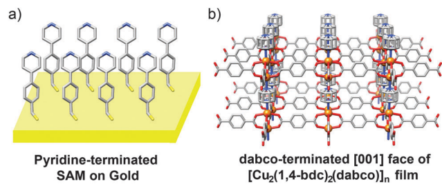
Fig. 24 Comparison of (a) an idealised self-assembled monolayer of PPMT on a gold surface and (b) the [001] face of [Cu 2 (1,4-bdc) 2 (dabco)] n , both of which present N-donor ligands for deposition of a MOF thin film. Both substrates can be surface functionalised with a layer of HKUST-1.
