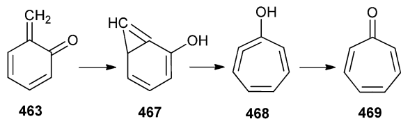
Scheme 102 Synthesis of tropone from o -QM.
