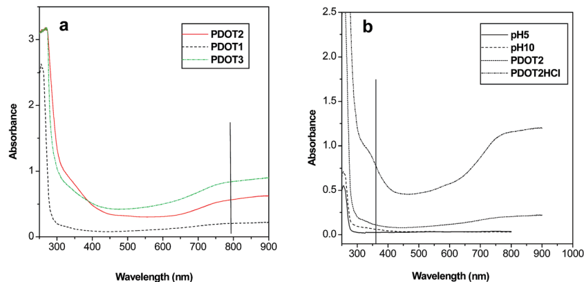
Fig. 3 UV-vis absorption spectra of PEDOT-PSS solutions at (a) different concentrations and at (b) different pH values.
