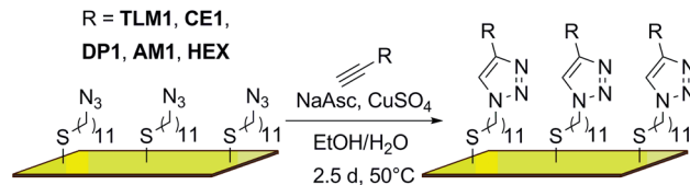
Scheme 2 Surface attachment of organic molecules via “click” chemistry ( \text{NaAsc} = sodium ascorbate).
