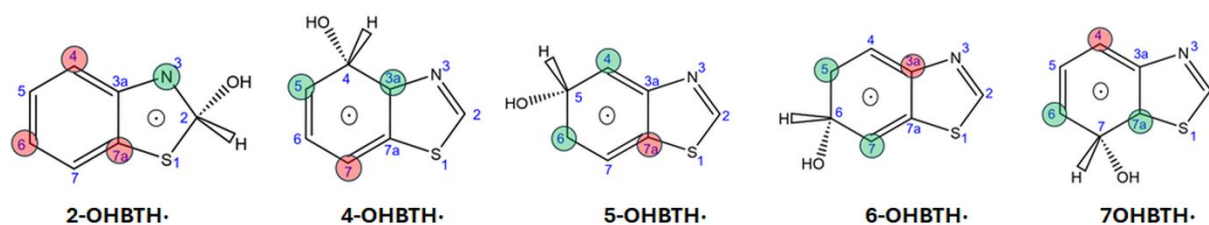
Figure 5. Oxygen attack sites in the intermediate radical n-OHBTH (n = 2, 4, 5, 6, 7). The green and red circles highlight the reactive and non-reactive sites of O 2 attack, respectively.
