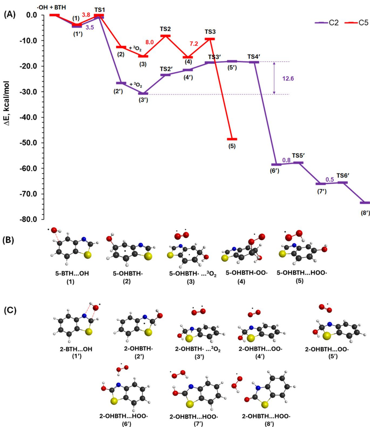
Figure 4. (A) Stationary points on the PESs of the reaction between BTH and the hydroxyl-radical. The method is (CDFT-B2PLYP/6-311++G**//B3LYP-D/6-311+G*). For the C5 attack, the stationary points are numbered (1) – (5), with transition states labeled TS1, TS2, and TS3 (in red). The C5 attack scenario also represents cases involving C4, C6, and C7 attacks. For the C2-attack, the stationary points are numbered (1) – (8') with transition states labeled TS1 – TS6' (in purple). Note: when zero-point energy corrections are applied in a simple harmonic approximation, the energies of transition states TS2', TS3' and TS4' become lower than those of the related stationary points. (B) Structures of the stationary points on the PES for the formation of 5-OHBTH. (C) Structures of the stationary points on the PES for the formation of 2-OHBTH. Note: transition state structures can be found in Fig. S9.
