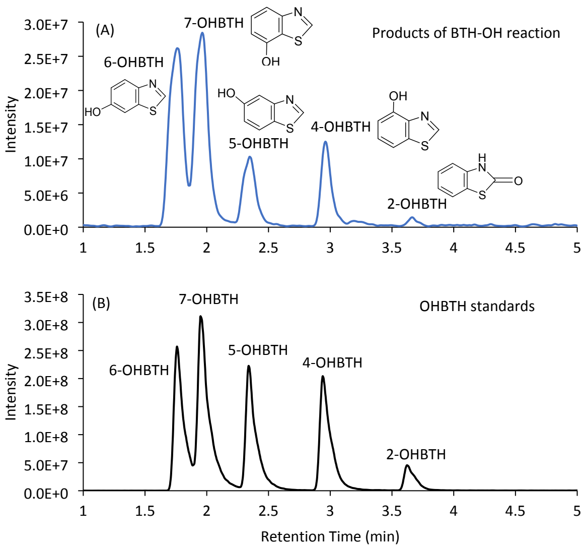
Figure 2. Extracted ion chromatograms (EIC) of BTH-OH reaction products for m/z 152 from TQD of (A) products of the reaction of OH with BTH and (B) OHBTH standards (500 ng/ml each) in 50:50 ACN/water.
