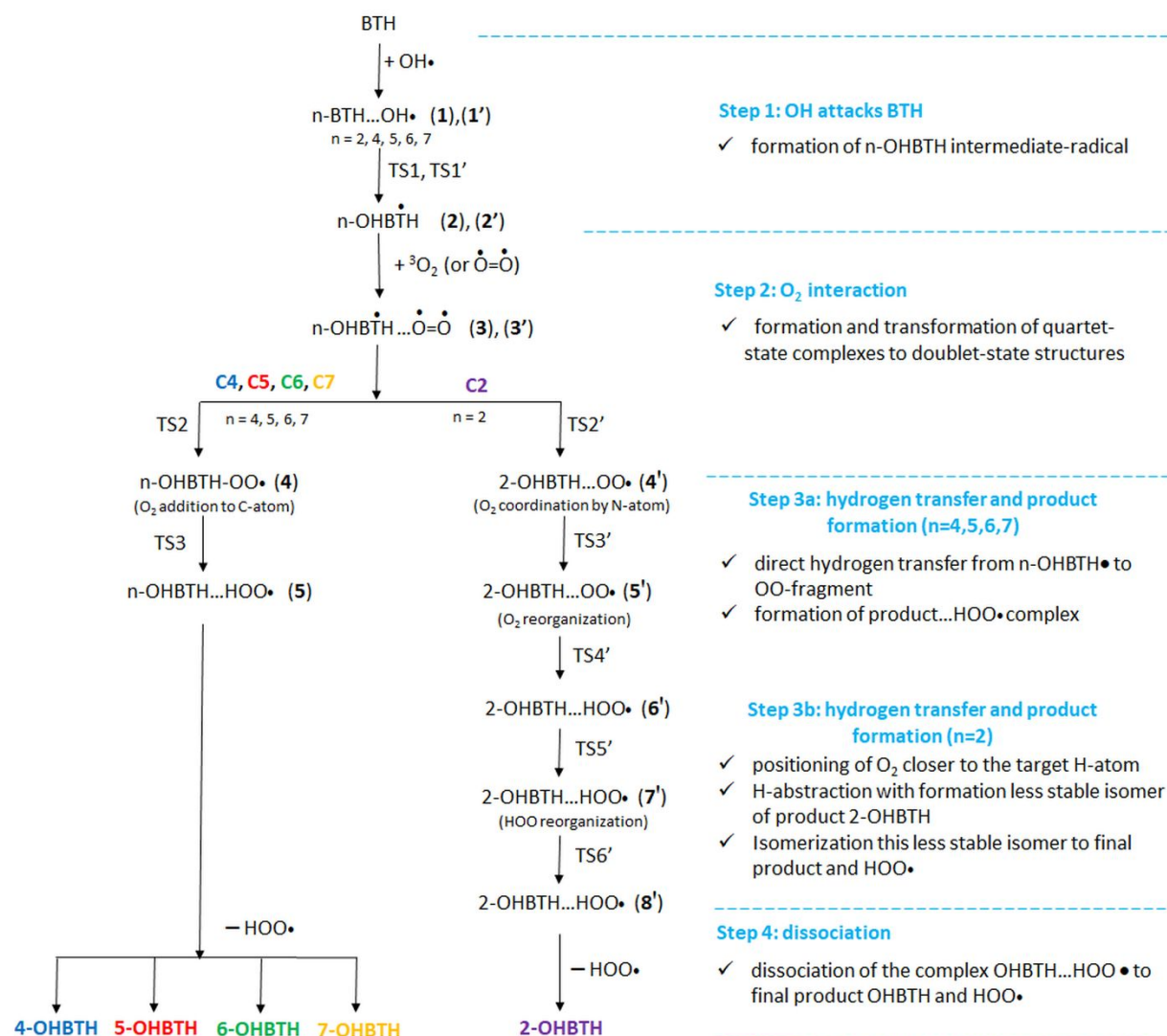
Figure 3. Proposed mechanism for the reaction of OH with BTH via the initial attack on different carbon sites.
