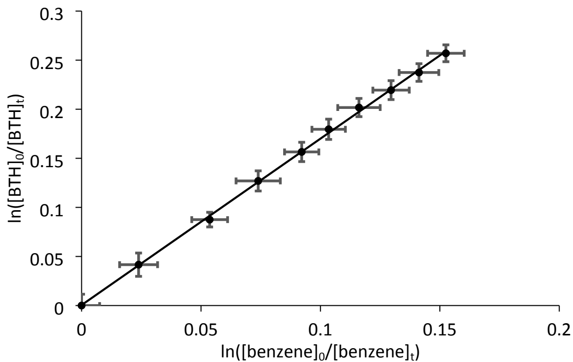
Figure 1. Typical relative rate data for the reactions of OH radicals with BTH and benzene at 298 K and 1 atm pressure in air.
