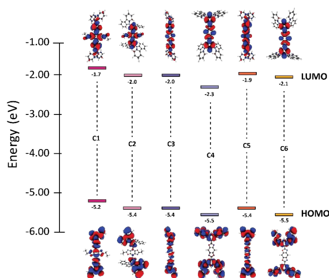
Figure 2. FMOs and electronic energy levels of C1-C6.
