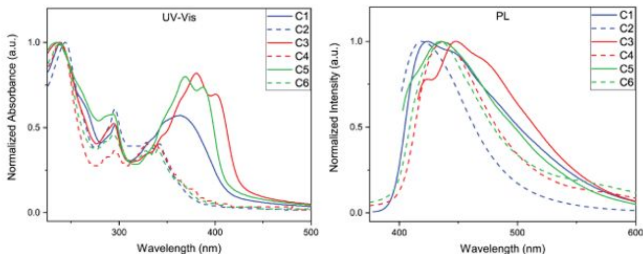
Figure 3. Steady-state absorbance spectra of C1-C6 in chloroform (left) at 0.01 gL -1 and photoluminescence spectra of C1-C6 thin-film (right).
