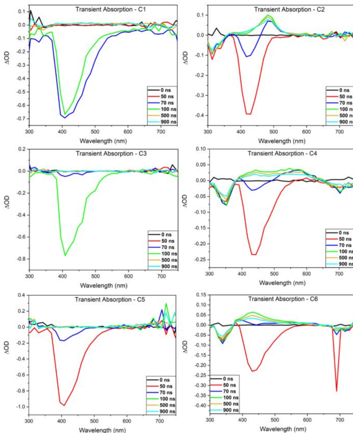
Figure 4. Nanosecond transient absorption spectra of the six BBOs.
