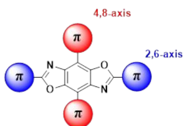
Figure 1. General structure of the BBO core. Conjugation can take part at the 2 and 6 positions (axis) or the 4,8 axis.
