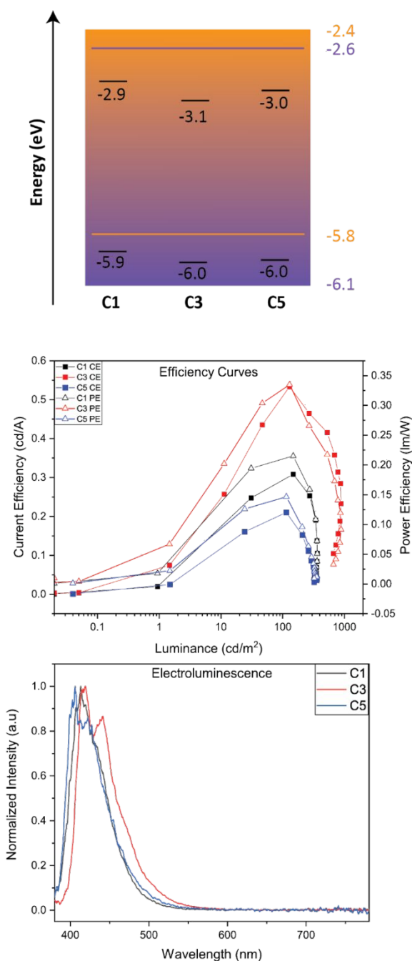
Figure 5. (top) Band diagram of active layer materials using BBO-based dopants. In purple are the HOMO/LUMO levels for 26DCzPPY while in orange is TCTA. (center) Power and current efficiency curves. (bottom) Normalized EL spectra.
