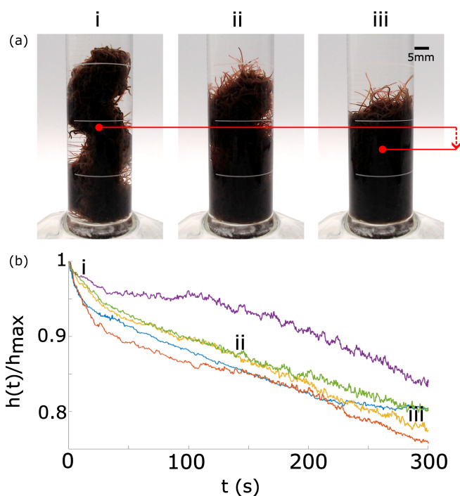
Fig. 14 Evolution of a worm blob from a rigid structure at high concentration of DO to a loosely entangled state in a lower concentration of DO. (a) The red dot depicts the centroid, which decreases over time as DO is consumed by the worms. Blackworms supplement respiration by disentangling their posterior segments and raising it upwards, emergently relaxing the structure. (b) The normalized height of the blob's centroid, \frac{h(t)}{h_{max}} , plotted as a function of time. Numbers in the time series correspond to the snapshots shown in (a). n = 5 trials. (Supplementary Movie S2)
