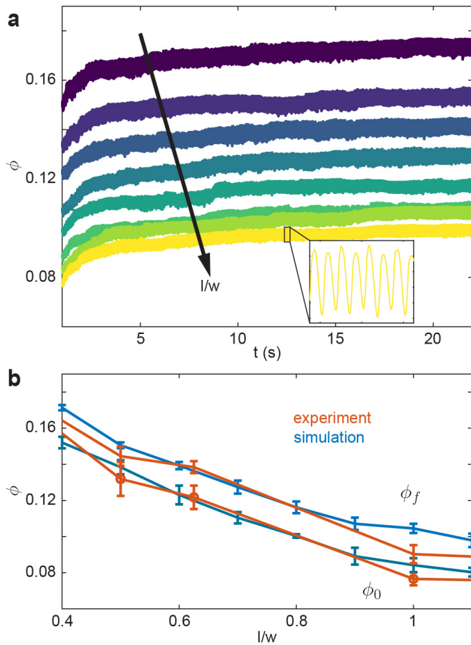
Fig. 3 Packing fraction and packing evolution as a function of smarticle aspect ratio. (a) \phi vs. time for various smarticles aspect ratios l/w \in [0.4, 1.1] . The inset is a zoomed in version of the data from l/w = 1.1 over a 0.25 s domain. (b) \phi as a function of aspect ratio in experiment (orange) and simulation (blue). The bottom two curves represent the volume fraction before activity was added to the system \phi_0 in both simulation and experiment. The top two curves are the volume fraction after external forcing \phi_f . The orange curves were taken from data used in Gravish et al. 10
