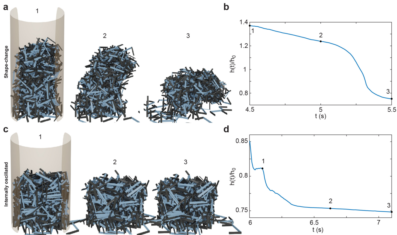
Fig. 10 Melting behavior for active procedures.(a,c) Renders of a shape-change trial and internally-oscillated trial, respectively, at three instances. (b,d) The z-plane center-of-mass (CoM) of the collective vs. time, where the three renders from (a,c) are indicated with black points.
