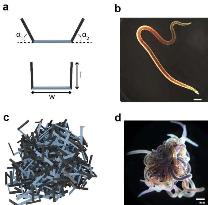
Fig. 1 Smarticles in simulation and biological analogy. (a) The coordinate system and size designations used for the smarticles. (b) An individual California blackworm ( Lumbriculus variegatus ). (c) An entangled pile of smarticles in simulation. (d) A group of 20 individual blackworms forming a physically-entangled blob.
