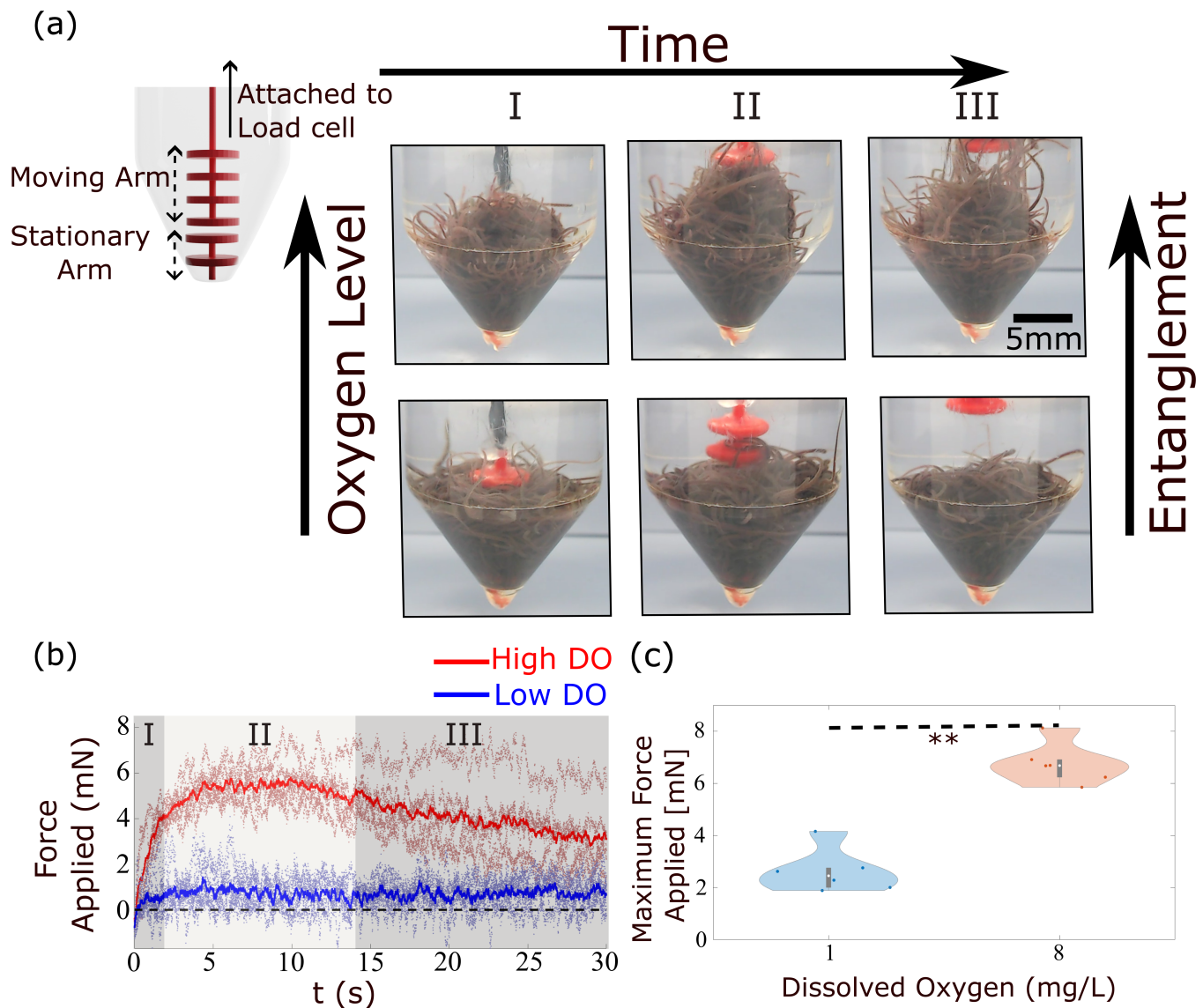
Fig. 17 Experimental setup for blackworms. (a) Two 3D-printed pieces were placed inside a conical tube: the lower stationary arm was fixed to the bottom to anchor the worms while the upper moving arm was attached to a load cell above. The load cell was attached onto a linear actuator, which allows the upper arm to move in the z-direction. 2g of worms ( N \sim 250 ) were added into the tube and mixed to allow an even distribution around the arms. The upper arm was gradually raised and the force was measured. The images show snapshots from trials with low DO concentration (bottom row) and high DO concentration (upper row), taken from successive epochs during the trial. Insets show zoomed-in images of column II. (b) Graph of force applied, in mN, on the load cell as a function of time, for low DO concentration (blue curve) and high DO concentration (red curve). The three epochs I-III in panel (a) correspond to the shaded regions in panel (b). The data points correspond to individual experimental runs and the solid curves are averages across trials. (c) Violin plot of maximum pulling force, in mN, vs. dissolved oxygen level. The solid rectangles indicate the interquartile range while the whiskers indicate the maximum and the minimum value of the distribution. The individual data points are plotted as dots. ** indicate a significance level of 1%. n = 6 trials for each DO levels.
