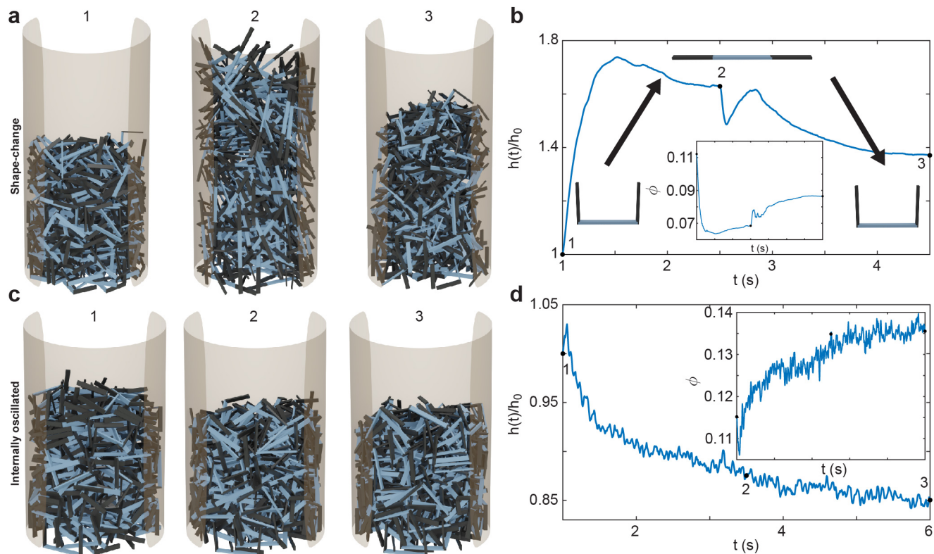
Fig. 4 Packing behavior distinctions between two different active procedures. (a) Renders of a shape-change trial at three instances. (b) The center-of-mass (CoM), \frac{h(t)}{h_0} , in the z-plane of the shape-change collective, the times of the renders in (1,2,3) are highlighted with black points [1s, 2.5s, 4.5s]. (c) Renders of an internally oscillated trial at three times. (d) The CoM in the z-plane of the internally-oscillated collective, the times of the renders in (1,2,3) are highlighted with black points [1s, 3.5s, 6s].
