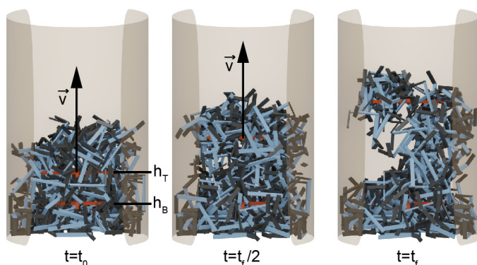
Fig. 12 Measuring force as a function of entanglement procedure. Two hooks, colored red, were embedded in an already entangled pile. The force necessary to raise the top hook out of the pile, at constant speed, was measured, while the bottom hook was kept fixed to anchor the pile.
