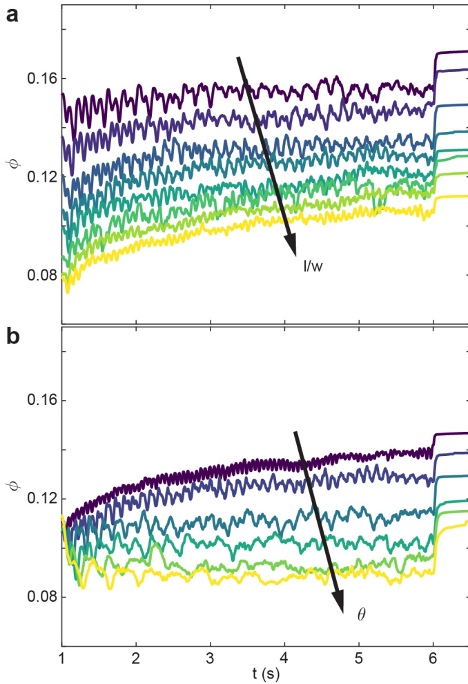
Fig. 6 Time evolution of volume fraction \phi for various l/w and \theta for the internally-oscillated procedure. (a) l/w is varied \in [0.4, 1.1] while \theta = 10^\circ is held constant. (b) \theta is varied \in [5^\circ, 30^\circ] while l/w = 0.7 is held constant.
