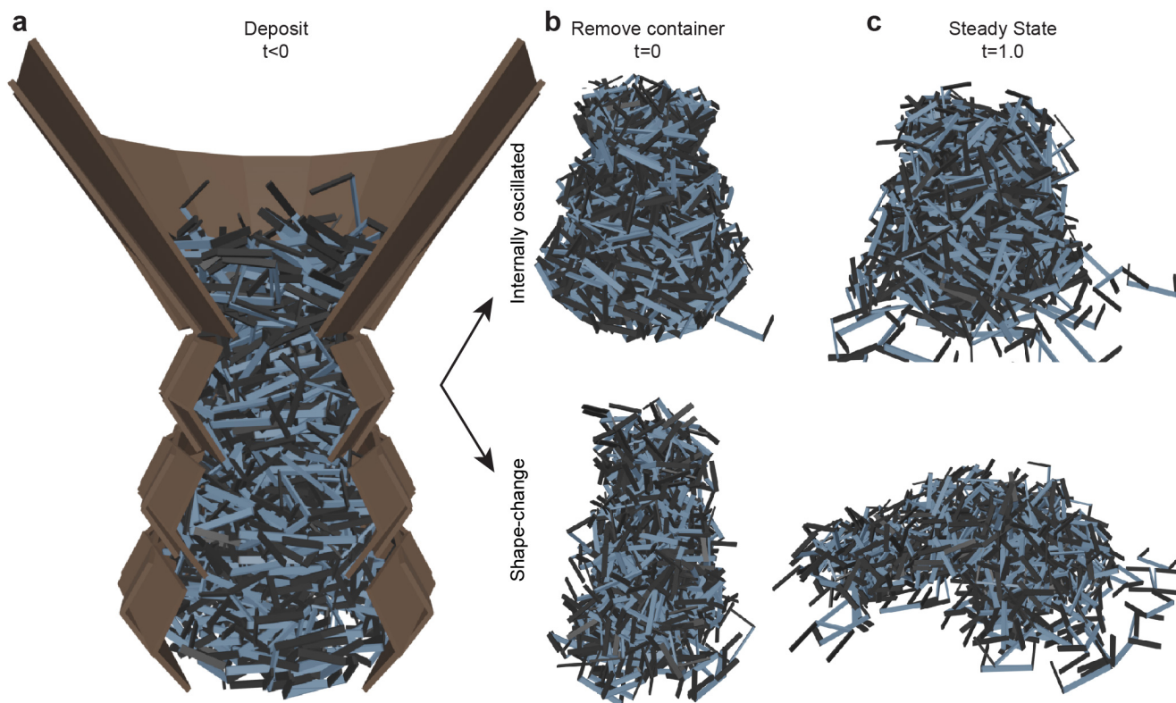
Fig. 11 Smarticle aggregate sculpting capabilities. (a) Particles are deposited in a three-tiered system at l/w = 0.8 with each tier smaller than the one below. In (b), after the activation state has occurred, (top is internally-oscillated at \theta = 10^\circ and bottom is the shape-change) the outer walls are removed. (c) The piles one second after the container is removed for the internally-oscillated (top) and shape-change (bottom) procedures. (Supplementary Movie S1)
