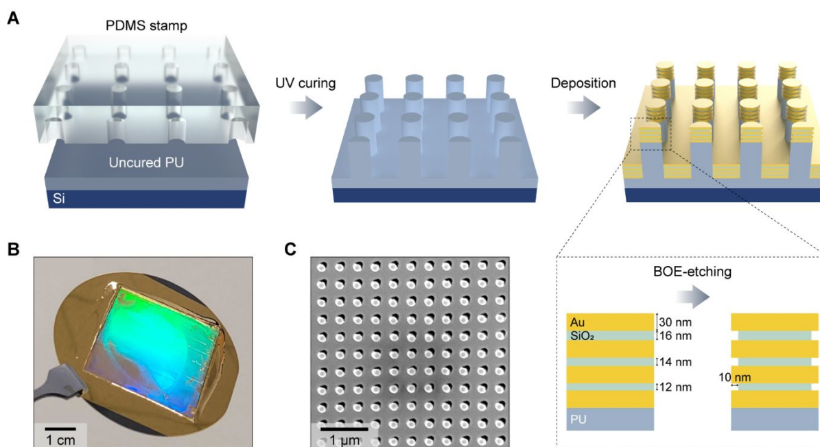
Fig. 1. Fabrication of 3D nanolaminate plasmonic crystals (NLPC) as a SERS substrate for dopamine (DA) sensing. (A) Schematic illustration of the fabrication process for a 3D NLPC SERS substrate. (B) Photographic and (C) top-view SEM images of a 3D NLPC SERS substrate.
