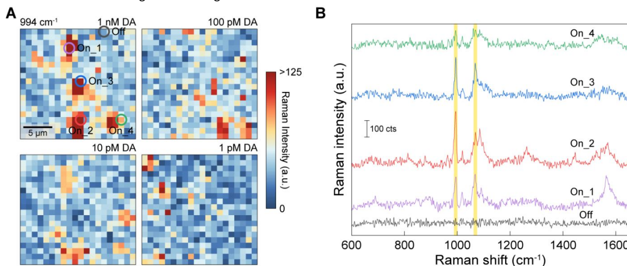
Fig. 5. SERS mapping results from the 3D NLPC-based DA-specific dual-recognition structures coupled with AuNPs using different concentrations of DA. (A) SERS mapping images using the intensity of the 3-MPBA peak at 994 cm -1 for different DA concentrations. (B) Raman spectra of four different "On" sites and one "Off" site. The origins of the spectra are depicted as circles in Fig. 5A.
