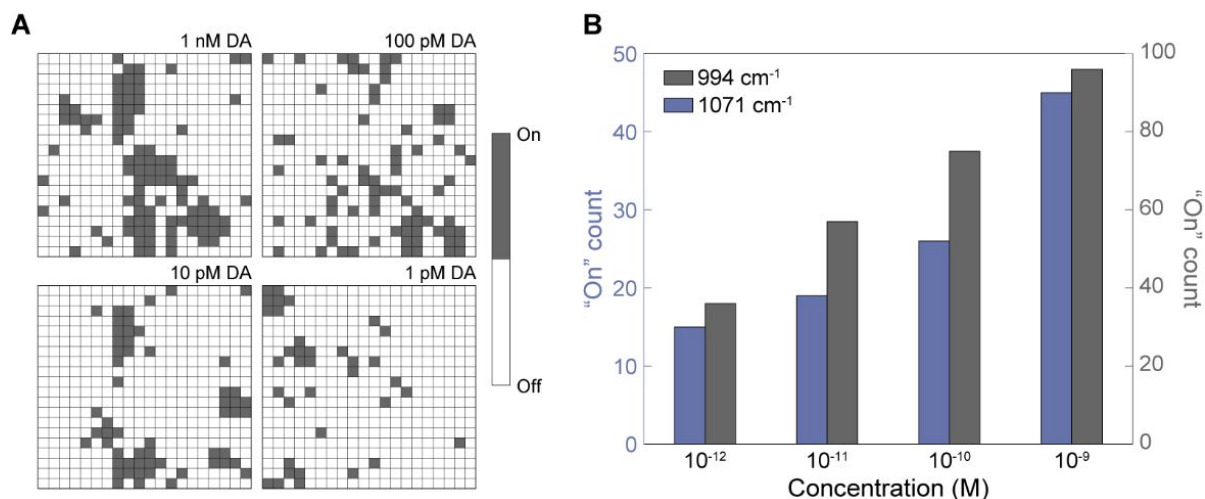
Fig. 6. Digital SERS sensing for the quantitative determination of DA. (A) Digital mapping images with different DA concentrations, converted from those in Fig. 5A. (B) Histogram of the total number of “On” spectra using two main peaks for 3-MPBA at 994 and 1071 \text{cm}^{-1} (the yellow lines in Fig. 5B).
