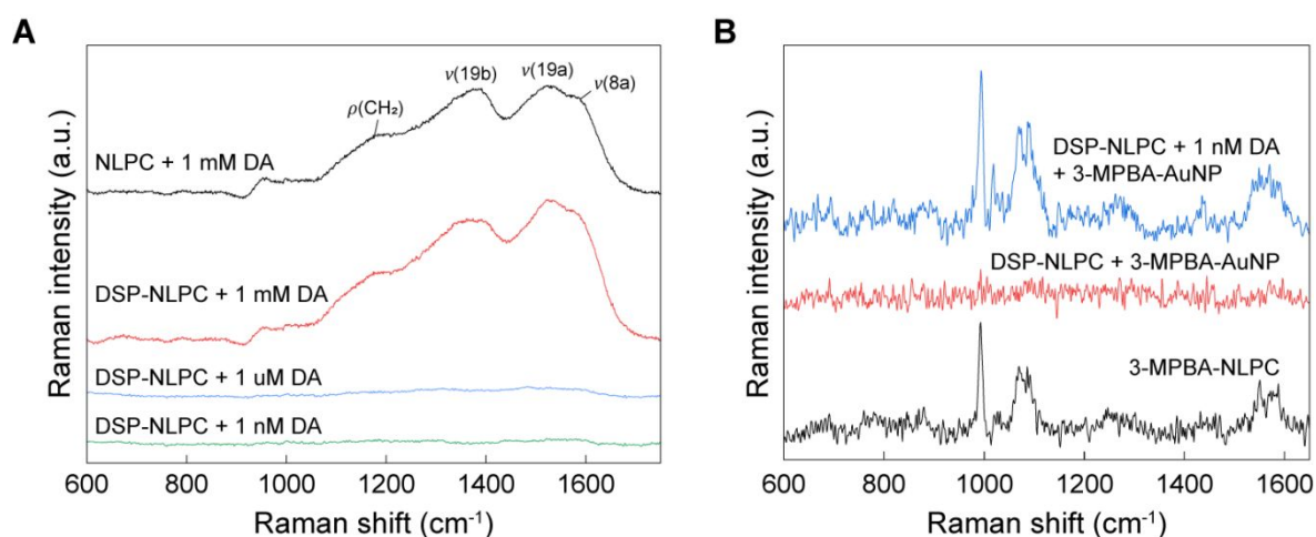
Fig. 4. 3D NLPC-based DA detection using label-free and Raman tag-labeled SERS sensing. (A) Raman spectra for DA on the NLPC substrates functionalized with and without DSP for label-free SERS sensing at different DA concentrations. (B) Raman spectrum for the DA-specific dual-recognition structure at 1 nM DA, compared with configurations without DA and/or Raman tag-conjugated AuNPs.
