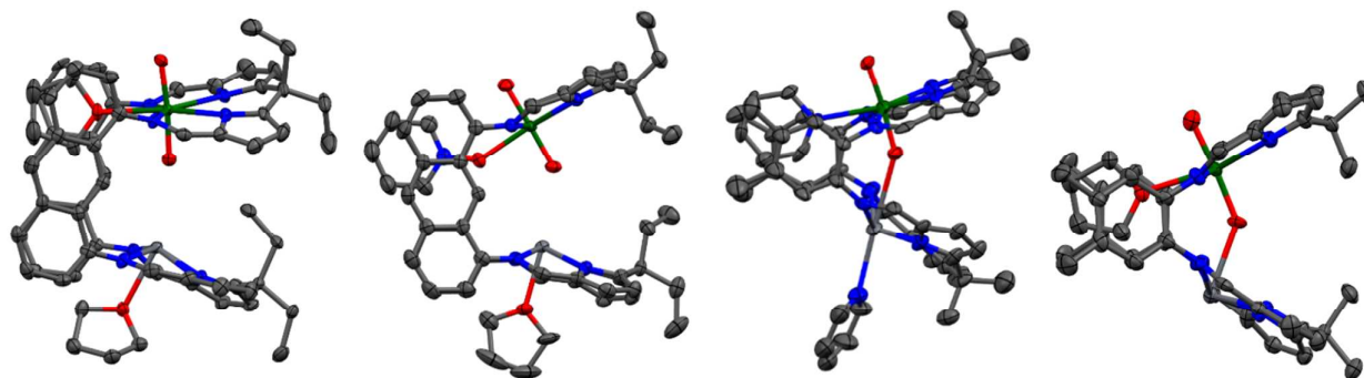
Figure 1: Solid-state structures of (a) 1(Pb)-THF ; (b) 2(Pb)-THF ; (c) 3(Pb)-py ; (d) 3(Pb)-THF . For clarity, all hydrogen atoms and solvent of crystallisation are omitted (displacement ellipsoids are drawn at 50% probability). Atom colours: green = uranium; blue = nitrogen; red = oxygen; light grey = Group 14 element; dark grey = carbon.
