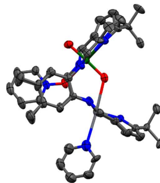
Figure 2: Solid state structure of 4(Pb)-py . For clarity, all hydrogen atoms are omitted (displacement ellipsoids are drawn at 50% probability). Atom colours: green = uranium; blue = nitrogen; red = oxygen; light grey = lead; dark grey = carbon.
