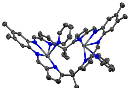
Figure 3: Solid state structure of 5 . For clarity, all hydrogen atoms are omitted (displacement ellipsoids are drawn at 50% probability). Atom colours: blue = nitrogen; light grey = lead; dark grey = carbon.
