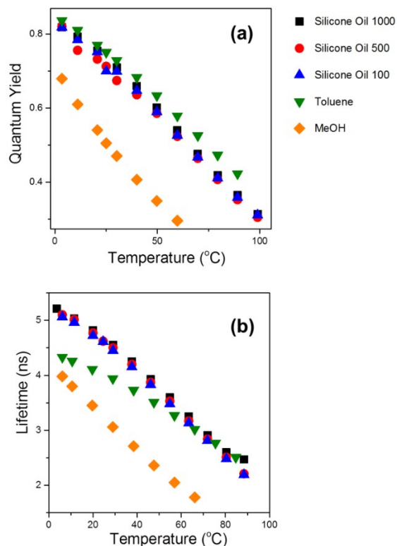
Figure 5. Fluorescence quantum yields (a) and fluorescence lifetimes (b) recorded for compound 2 in various solvents upon a temperature change between 3.5 and 99 °C.
