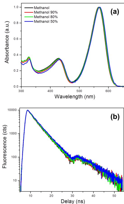
Figure 6. Absorbance spectra (a) and fluorescence time resolved decay traces (b) recorded for compound 2 in methanol/glycerol mixtures at 25 °C. The corresponding quantum yields were 0.57 (methanol), 0.61 (10% glycerol), 0.63 (20% glycerol) and 0.71 (50% glycerol)
