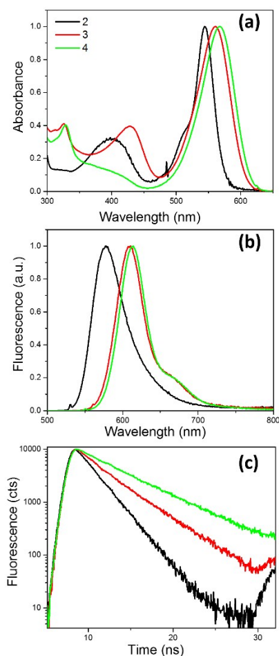
Figure 2. (a) Absorption, (b) fluorescence spectra and (c) time-resolved fluorescence decay traces recorded for 2-4 in acetonitrile solutions at 25 °C. Excitation wavelength 560 nm.
