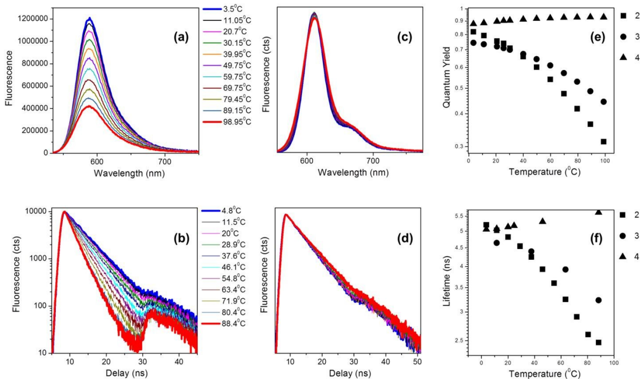
Figure 3. Fluorescence spectra (a, c) and time resolved fluorescence decays (b, d) of compounds 2 (a, b) and 4 (c, d) in Silicone oil 1000 recorded upon a temperature change between 3.5 and 99 °C. Quantum yields (e) and fluorescence lifetimes (f) recorded for compounds 2 , 3 and 4 in Silicone oil 1000 upon a temperature change between 3.5 and 99 °C. Excitation wavelength 560 nm, detection wavelength 589 nm (b) and 612 nm (d).
