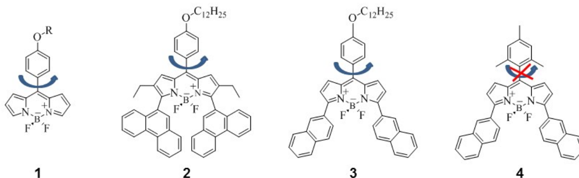
Figure 1. Chemical structure of phenyl-BODIPY derivatives under study
