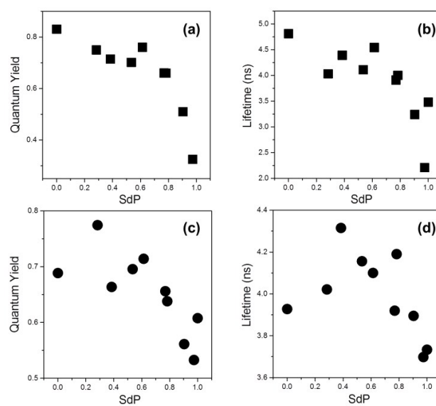
Figure 7. Fluorescence quantum yields (a, c) and fluorescence lifetimes (b, d) recorded for compound 2 (a, b) and 3 (c, d) in solvents of variable polarity at room temperature. The SdP parameters for all solvents used were taken from ref 26 and are listed in the SI, Table S4
