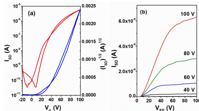
Fig. 6 The transfer (a) and output (b) profiles of 8 measured in solution-processed OFET under ambient conditions.
