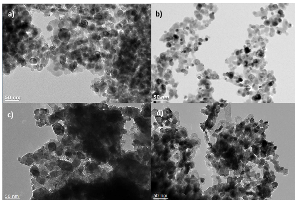
Figure 4. High resolution TEM micrographs of a) 1 , b) 4 , c) 5e and d) 5f at 50 000 \times magnification.
