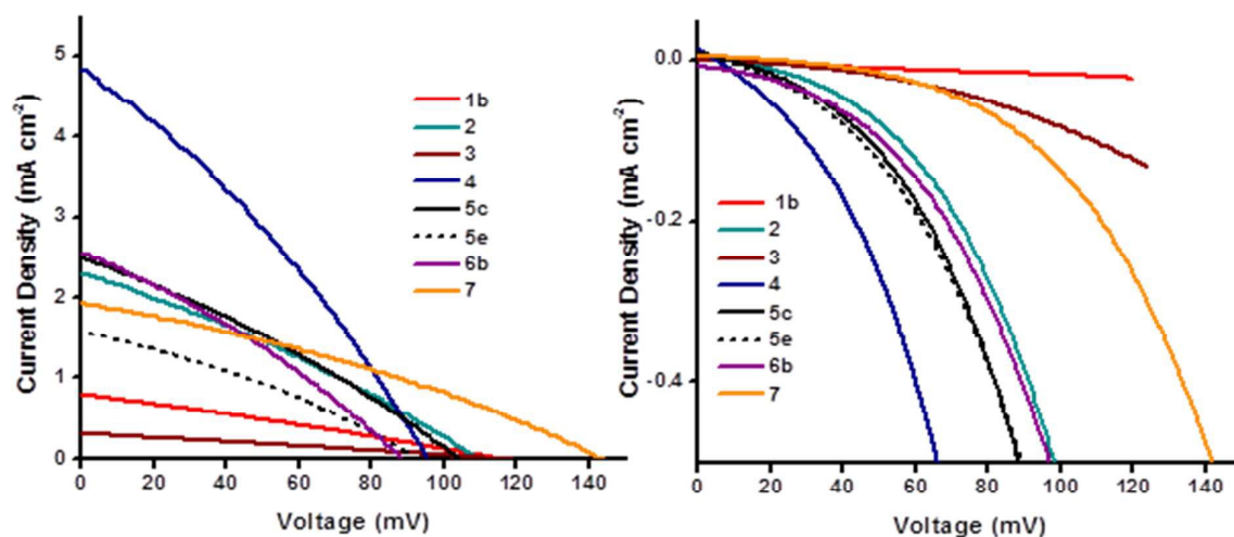
Figure 9. Plot of current density vs. voltage curves (a) under AM1.5 illumination and (b) in the dark for the NiO DSCs.
