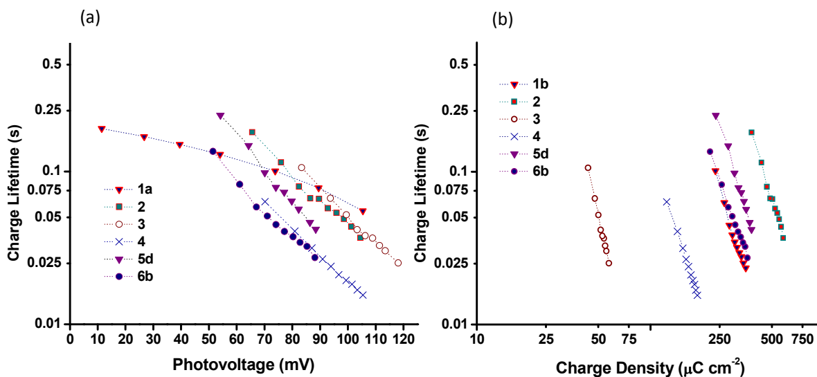
Figure 10. Plots of charge lifetime vs. (a) photovoltage and (b) charge density.
