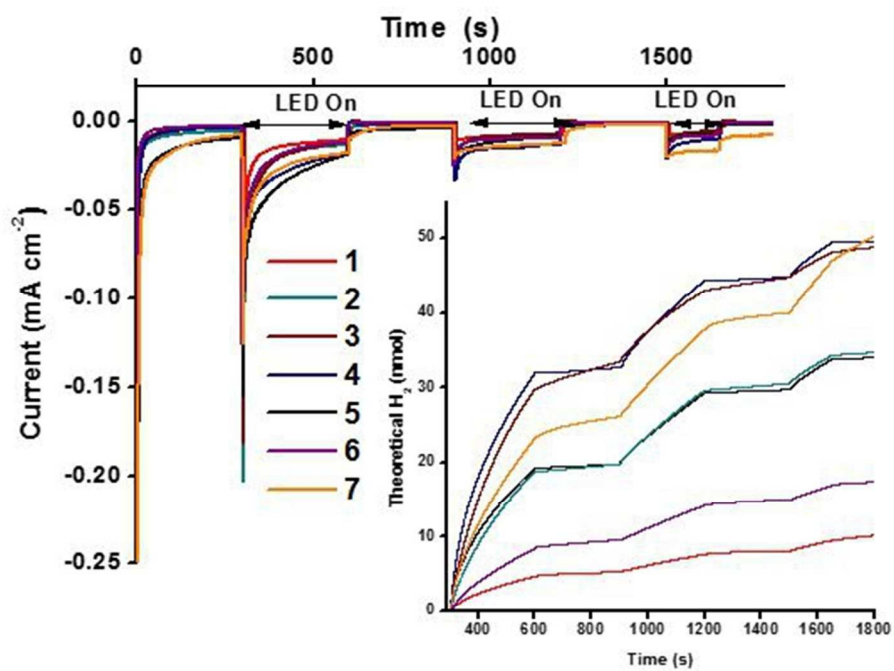
Summary of photocurrent vs. time and (inset) total theoretical H 2 generated for the 7 different NiO electrodes compared in this study. 157x115mm (96 x 96 DPI)
