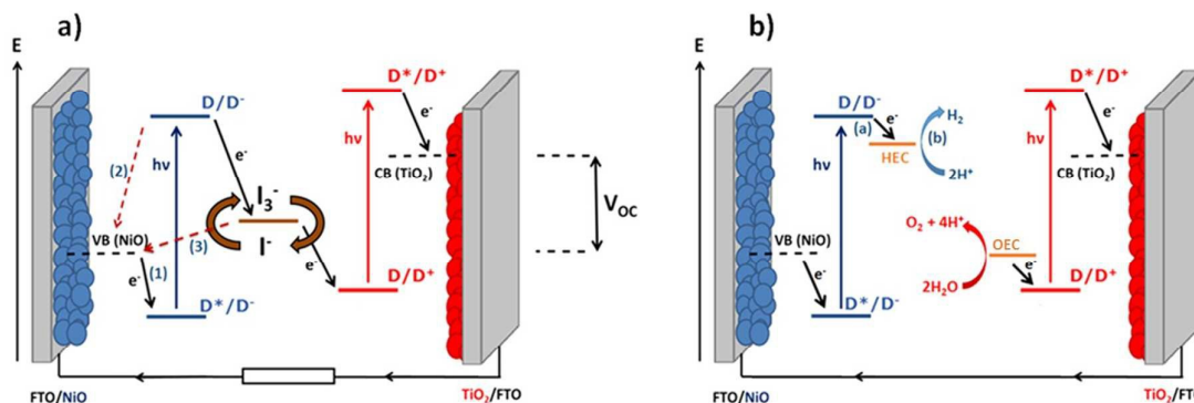
Figure 1. Schematic illustration of (a) a tandem dye-sensitized solar cell and (b) a dye-sensitized photoelectrosynthetic cell. (VB: Valence Band; CB: Conduction Band; HEC: Hydrogen Evolution Catalyst; OEC: Oxygen Evolution Catalyst).
