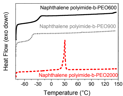
Fig. 3 DSC curves for Naphthalene polyimides-b-PEO600 (black solid line), naphthalene polyimide-b-PEO900 (grey dot line) and Naphthalene polyimide-b-PEO2000 (red dashed line) at 10\text{ }^{\circ}\text{C}\cdot\text{min}^{-1} .
