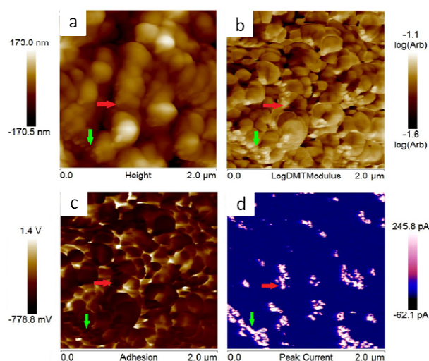
Fig. 6 AFM images collected in the PeakForce TUNA mode, using a DC sample bias of 1 V on sample Naphthalene polyimide-b-PEO600 loaded with 15 wt% of carbon black. (a) Topography, (b) elastic modulus in log scale, (c) adhesion force and (d) peak current images. The red and green arrows are pointing on the same domains in all four pictures.
