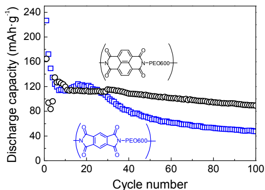
Fig. 8 Discharge capacities versus cycle number for Pyromellitic polyimide-b-PEO600 ( \square ) and Naphthalene polyimide-b-PEO600 ( \circ ) at 1\text{Li}^+/5\text{h} rate.
