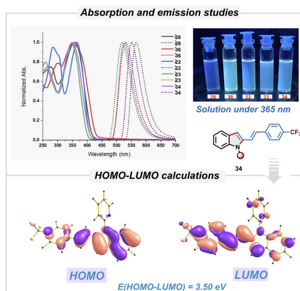
Scheme 5 Photophysical studies.
