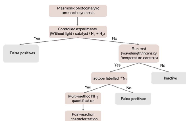
Fig. 13 Decision tree for artefact exclusion in plasmonic photocatalysis.
