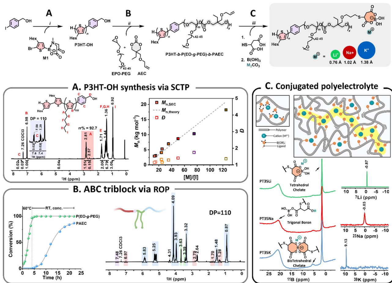
Fig. 1 Synthetic scheme for (A) SCTP synthesis of P3HT-OH macroinitiators for (B) chain growth to form ABC-triblock polymers in one-pot, which are converted to (C) polyelectrolytes via thiol-ene chemistry and alkali metal borate formation. For (A), ^1\text{H} NMR spectra ( \text{CDCl}_3 ) highlights regioregularity ( rr ) and DP determination for P3HT-OH ( DP = 110 ) with control over M_n achieved by the M1-to-iodobenzyl alcohol initiator ratio. For (B), conversion time showing ROP of EPO-PEG to P(EPO- g -PEG) (green) at elevated temperatures followed by AEC ROP to PAEC (blue) under cooled and concentrated reaction conditions to yield isolated products with representative ^1\text{H} NMR ( \text{CDCl}_3 ) shown. For CBEs (C), ^{11}\text{B} ( ^1\text{H} ) NMR spectra ( \text{DMSO-}d_6 ) showing borate environments alongside ^7\text{Li} , ^{23}\text{Na} or ^{39}\text{K} NMR spectra for PT35Li, PT35Na and PT35K (P3HT DP = 35 ), respectively confirming single cation environments.
