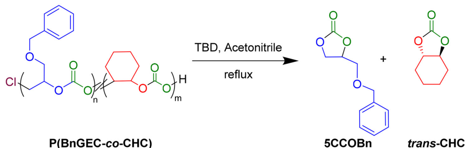
Scheme 3 Depolymerization of P(BnGEC-co-CHC) terpolymer using 1,5,7-triazabicyclo[4.4.0]dec-5-ene (TBD).
