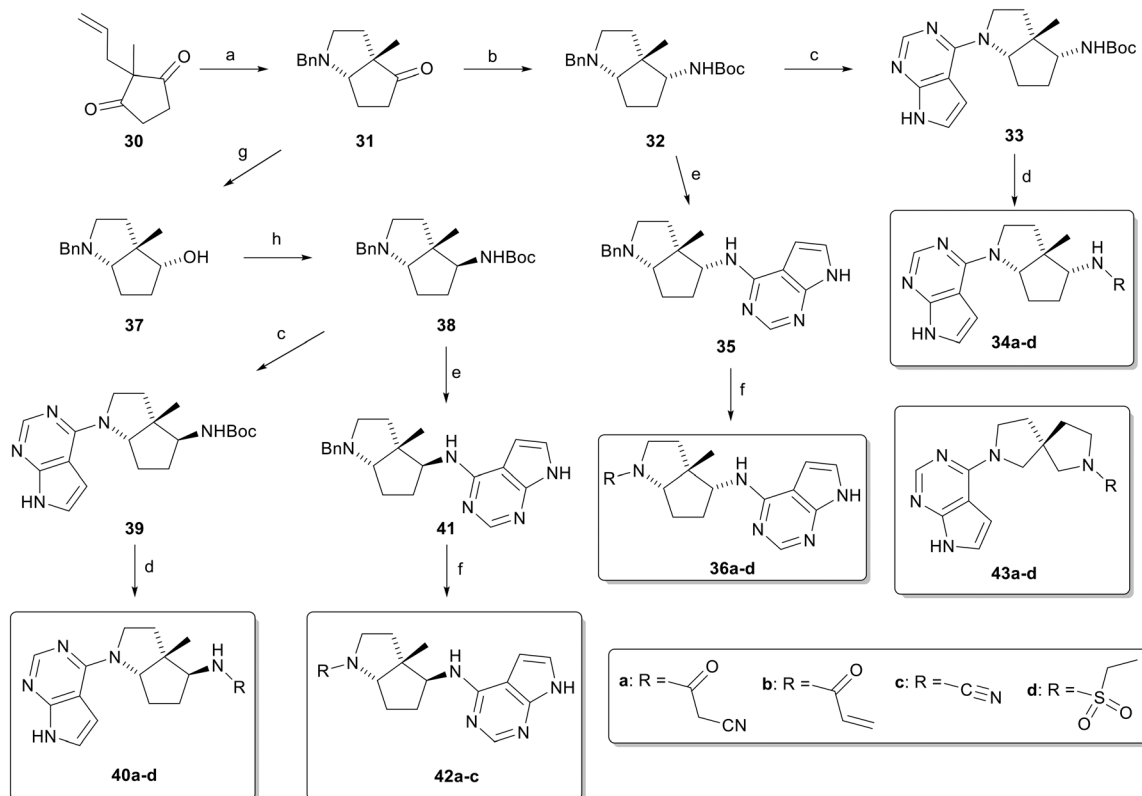
Scheme 2 Synthesis of deconstructed triquinazaine scaffolds. Conditions: a) i) \text{O}_3 , \text{DCM}/\text{MeOH} , 30 min, then \text{DMS} , 17 h, -78^\circ\text{C} to 22^\circ\text{C} , ii) \text{BnNH}_2 , \text{AcOH} , \text{CH}_2\text{Cl}_2 , 4 Å MS, 22^\circ\text{C} , 1 h, then \text{NaBH}(\text{OAc})_3 , 22^\circ\text{C} , 14 h, 61%; b) i) ammonium acetate, \text{NaBH}_3\text{CN} , \text{MeOH} , 50^\circ\text{C} , 19 h, ii) \text{Boc}_2\text{O} , \text{Et}_3\text{N} , \text{CH}_2\text{Cl}_2 , 22^\circ\text{C} , 1 h, 63%; c) i) cat. \text{Pd}/\text{C} , \text{H}_2 (1 atm.), \text{AcOH} , \text{MeOH} , 22^\circ\text{C} , 30 min, ii) 6-chloro-7-deazapurine, \text{K}_3\text{PO}_4 , t\text{-BuOH}/\text{H}_2\text{O} , 120^\circ\text{C} , 18 h ( 33 : 92%, 39 : 77%); d) i) \text{CF}_3\text{CO}_2\text{H} , \text{CH}_2\text{Cl}_2 , 22^\circ\text{C} , 1 h; ii) for 34a and 40a : 1-cyanoacetyl-3,5-dimethylpyrazole, \text{DIPEA} , \text{MeCN} , 75^\circ\text{C} , 4 h ( 34a : 95%, 40a : 69%), for 34b , 45d , 40b , 40d : coupling acyl chloride, \text{NaHCO}_3 , \text{DIPEA} , \text{CH}_2\text{Cl}_2 , 0^\circ\text{C} to 22^\circ\text{C} ( 34b : 46%, 34d : 76%, 40b : 31%, 40d : 20%), for 34c , 40c : cyanogen bromide, \text{NaHCO}_3 , \text{MeOH} , 0 – 22^\circ\text{C} , ( 34c : 15%, 40c : 14%); e) i) \text{DCM}/\text{TFA} , 22^\circ\text{C} , 1 h, ii) \text{K}_3\text{PO}_4 , t\text{-BuOH}/\text{H}_2\text{O} , 6-chloro-7-deazapurine, 80^\circ\text{C} , 6 days ( 35 : 76%, 2 steps), for 41 : i) \text{DCM}/\text{TFA} , 22^\circ\text{C} , 1 h, ii) \text{K}_3\text{PO}_4 , t\text{-BuOH}/\text{H}_2\text{O} , 6-chloro-7-deazapurine, 120^\circ\text{C} , 72 h, 50%; f) i) \text{Pd}(\text{OH})_2 , \text{MeOH}/\text{THF} , 22^\circ\text{C} , 2 h, ii) for 36a , 42a : 1-cyanoacetyl-3,5-dimethylpyrazole, \text{DIPEA} , \text{MeCN} , 75^\circ\text{C} , 4 h ( 36a : 21%, 42a : 36%), for 36d , 42b : coupling acyl chloride, \text{NaHCO}_3 , \text{DIPEA} , \text{CH}_2\text{Cl}_2 , 0^\circ\text{C} to 22^\circ\text{C} ( 36b : 17%, 36d : 18%, 42b : 28%), for 36c , 42c : cyanogen bromide, \text{NaHCO}_3 , \text{MeOH} , 0 – 22^\circ\text{C} , ( 36c : 77%, 42c : 42%); special case 36b : i) \text{Boc}_2\text{O} , \text{CH}_2\text{Cl}_2 , \text{DMAP} , 22^\circ\text{C} , 2 h, ii) \text{Pd}(\text{OH})_2 , \text{MeOH}/\text{THF} , 22^\circ\text{C} , 2 h, iii) acryloyl chloride, \text{NaHCO}_3 , \text{DIPEA} , \text{CH}_2\text{Cl}_2 , iv) \text{TFA} , \text{DCM} , 0^\circ\text{C} to 22^\circ\text{C} , 17%; g) \text{NaBH}_4 , \text{MeOH} , 0 – 22^\circ\text{C} , 45 min, 92%; h) i) \text{DPPA} , \text{DIAD} , \text{PPh}_3 , \text{THF} , 0 – 22^\circ\text{C} , 4 h, then \text{PPh}_3 , \text{H}_2\text{O} , 22^\circ\text{C} , 16 h, ii) \text{CH}_2\text{Cl}_2 , \text{Boc}_2\text{O} , \text{Et}_3\text{N} , 0 – 22^\circ\text{C} , 1 h, 46%.
