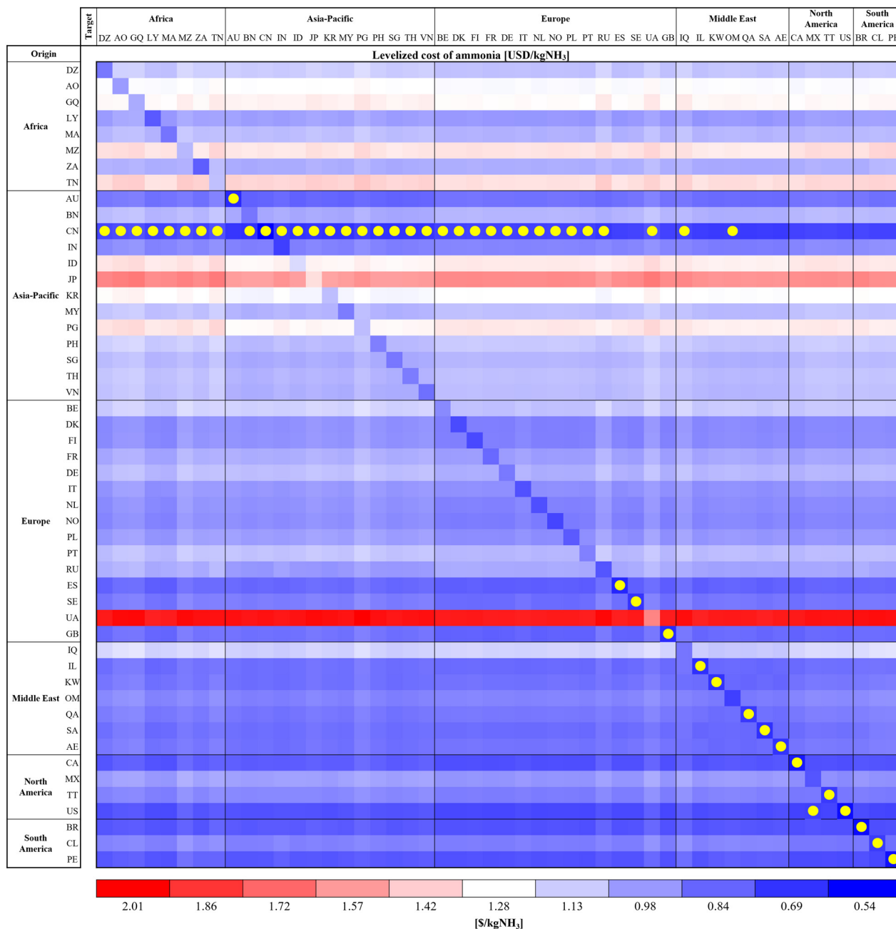
Fig. 14 Green NH 3 inter-country cost [$/kgNH 3 ]. Note that, EG, NA, NG, KZ, TM, UZ, AZ, CZ, BO, TR, IR, AR, and VE have been excluded for clearer visualization due to their out-ranged FCR, source availability, and their landlocked location. The diagonal line represents the domestic production cases. Yellow dot indicates the lowest origin country option for the corresponding target country.
