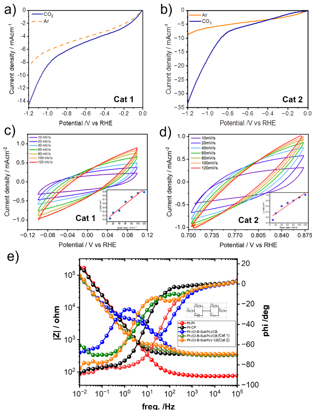
Fig. 3 (a) LSV curves at a scan rate of 30 \text{ mV s}^{-1} (Cl-B-SubPc)/CB (800 °C, Cat 1 )/CB WEs with Ar and \text{CO}_2 saturation 0.1 M \text{CsHCO}_3 . (b) LSV curves at a scan rate of 30 \text{ mV s}^{-1} (Cl-B-SubPc)/CB (1000 °C, Cat 2 ) WEs with Ar and \text{CO}_2 saturation 0.1 M \text{CsHCO}_3 . (c) Cyclic voltammograms of (Cl-B-SubPc)/CB (800 °C, Cat 1 ) at different sweep rates of 10, 20, 40, 60, 80, 100, and 120 \text{ mV s}^{-1} in 0.1 M \text{CsHCO}_3 and a linear plot of capacitive current versus scan rate. (d) Cyclic voltammograms of (Cl-B-SubPc)/CB (1000 °C, Cat 2 ) at different sweep rates of 10, 20, 40, 60, 80, 100, and 120 \text{ mV s}^{-1} in 0.1 M \text{CsHCO}_3 and a linear plot of capacitive current versus scan rate. (e) Bode plot recorded via electrochemical impedance spectroscopy of (Cl-B-SubPc)/CB, (Cl-B-SubPc)/CB (800 °C, Cat 1 ), and (Cl-B-SubPc)/CB (1000 °C, Cat 2 ) catalyst modified carbon paper electrode in the frequency range of 1 \times 10^{-2} \text{ Hz} to 1 \times 10^5 \text{ Hz} with a perturbation amplitude of 10 mV.
