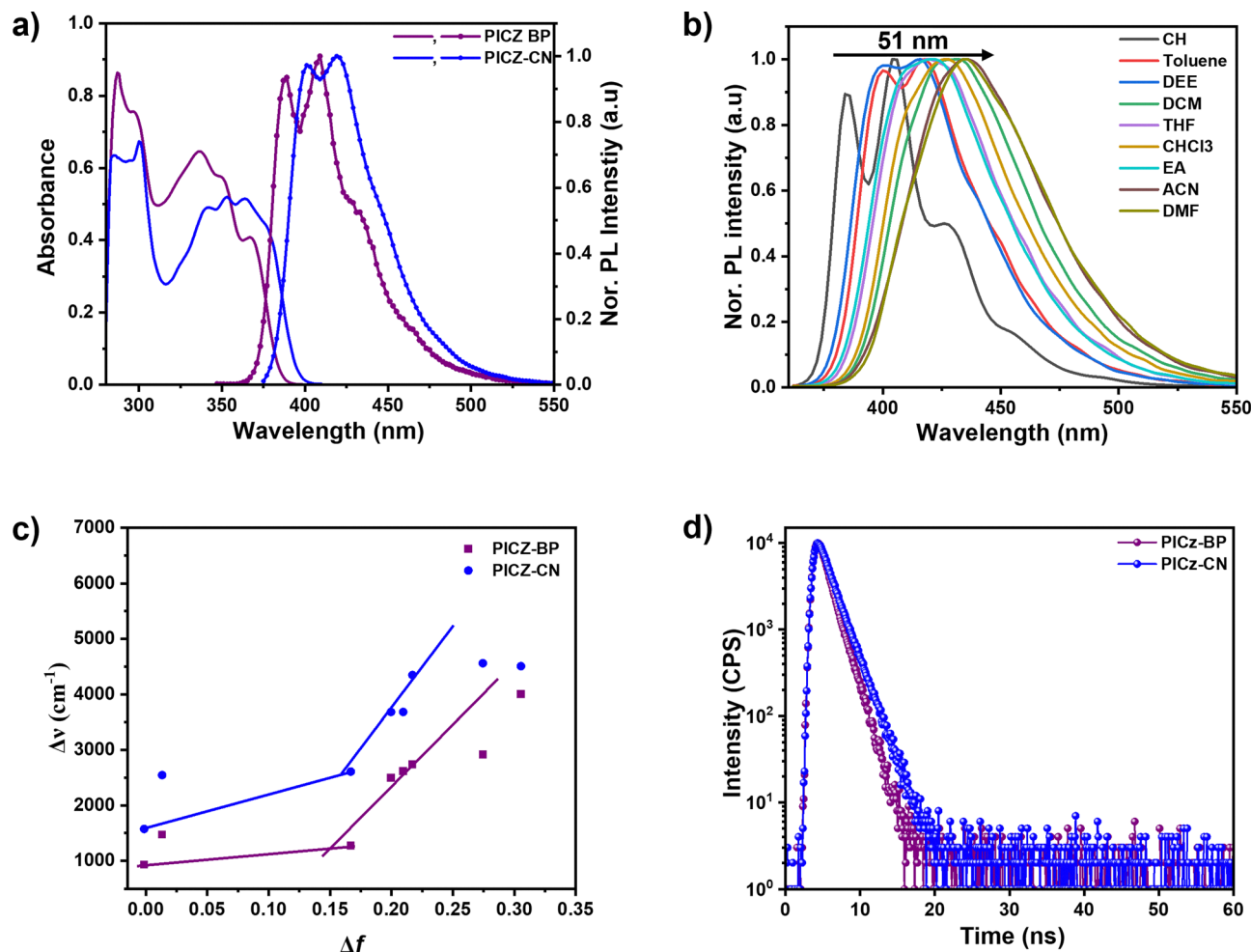
Fig. 3 (a) Absorption and emission spectra for the compounds in dilute toluene solution; (b) solvatochromic studies for the compound PICz-CN ; (c) Lippert–Mataga plot; (d) Lifetime decay curve.
