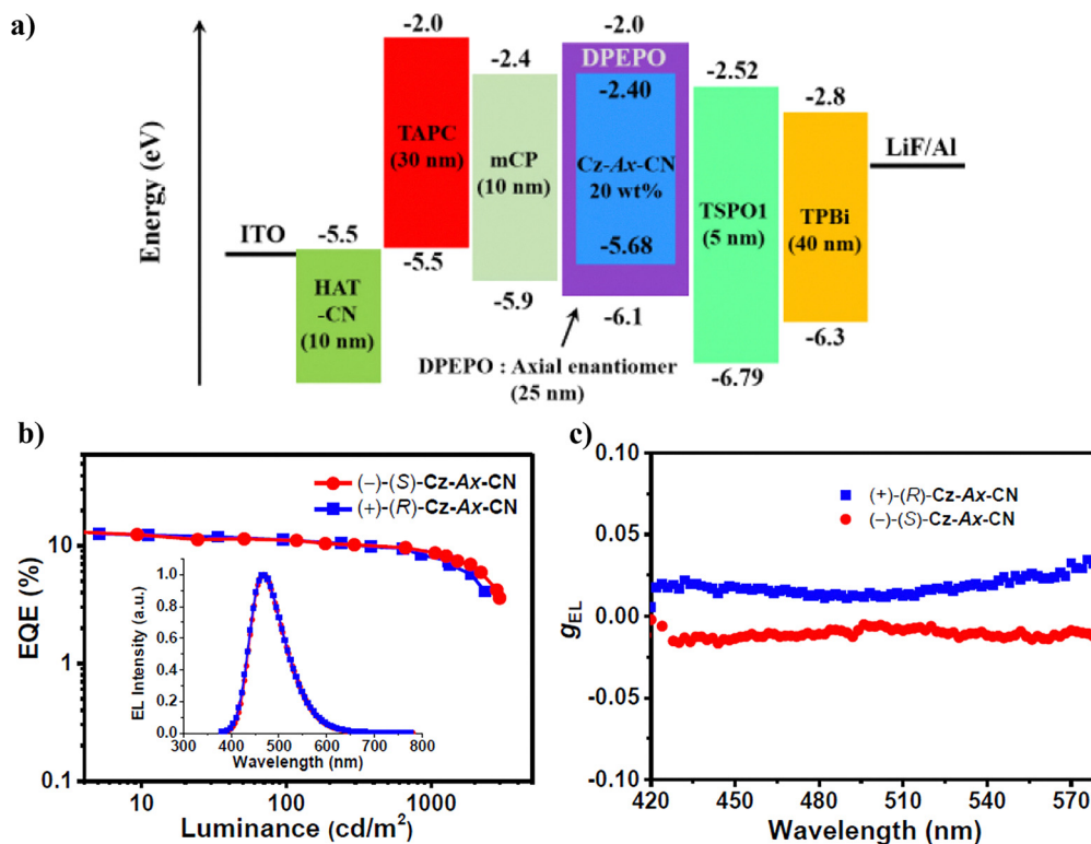
Fig. 17 (a) The energy diagram of CP-OLEDs based on (-)-(S)- 5 and (+)-(R)- 5 . (b) EQE–luminance characteristics. Inset: EL spectra of the devices at 6 V. (c) The g_{\text{EL}} values of the devices as a function of emission wavelength. Reproduced with permission from ref. 32. Copyright 2020, Wiley-VCH.
