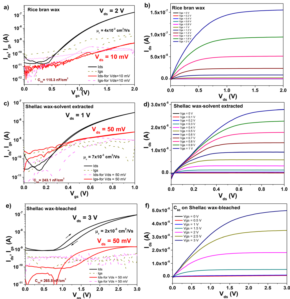
Fig. 14 (a) Transfer and (b) output characteristics of an OFET with C 60 semiconductor and rice bran wax dielectric on plain aluminum gate electrode; (c) transfer and (d) output characteristics of an OFET with C 60 semiconductor and solvent extracted shellac wax dielectric on plain aluminum gate electrode; (e) transfer and (f) output characteristics of an OFET with C 60 semiconductor and bleached shellac wax dielectric on plain aluminum gate electrode.
