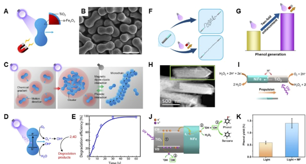
Fig. 2 Design, structure, and photocatalytic performance of TiO 2 /α-Fe 2 O 3 microrobots and TiO 2 /NiFe nanomotors. (A) Schematic illustration of TiO 2 /α-Fe 2 O 3 microrobots with light- and magnetically driven motion. (B) SEM image of peanut-shaped α-Fe 2 O 3 particles, scale bar 2 μm. (C) Self-assembly behaviour under chemical gradients and magnetic dipole–dipole interactions forming clusters and microchains. (D) Photocatalytic mechanism of dichlorophenoxyacetic acid (2,4-D) degradation via ROS generation mediated by UV light. (E) Graph showing time-dependent degradation efficiency of 2,4-D, reaching 97% in 30 minutes. Adapted with permission from Nature Communications , ref. 48 Copyright©2023. This is an open access article distributed under the terms of the Creative Commons CC BY license. (F) Schematic illustrating the motion behaviour of TiO 2 /NiFe nanomotors under UV light and magnetic fields. (G) Representation of improved photocatalytic phenol generation by the combined effects of light and magnetic fields. (H) STEM image of TiO 2 /NiFe nanomotors. (I) Photocatalytic propulsion mechanism of TiO 2 /NiFe nanomotors mediated by UV light, driven by electron transfer and H 2 O 2 decomposition. (J) UV light-induced electron excitation in TiO 2 and charge transfer to NiFe, generating ROS that oxidize benzene to phenol. (K) Phenol yield comparison under light and light + magnetic field conditions, showing enhanced performance. Reprinted with permission from ACS Applied Materials & Interfaces , ref. 50 (ACS) Copyright©2023. ( https://pubs.acs.org/doi/10.1021/acsami.4c03905 ). Readers are advised that any requests for additional permissions relating to the extracted material must be addressed directly to ACS.
