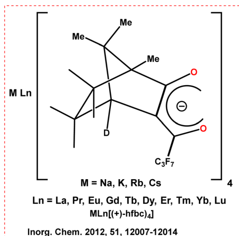
Scheme 9 Chemical structures of the ligands and Ln complexes (\text{MLn}(\text{hfbc})_4)_4 . 60
