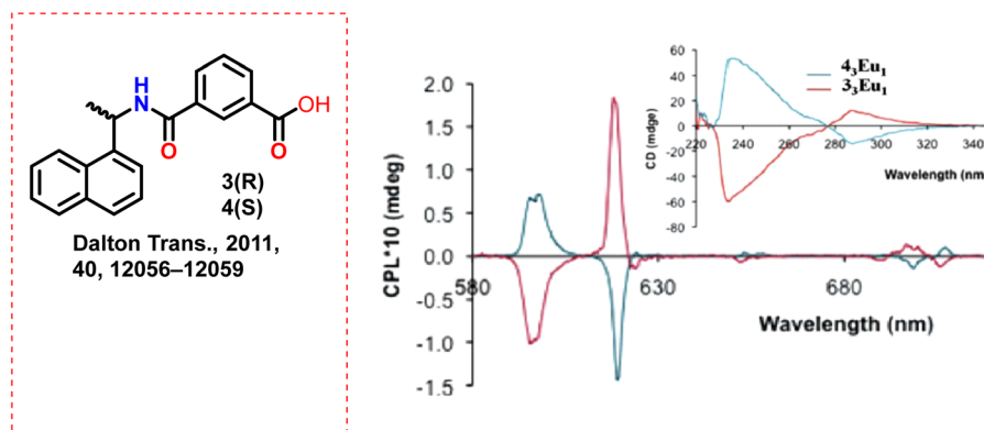
Scheme 19 (Left) Chemical structures of ligands 3 and 4. 64 (Right) Eu(III) circular polarised emission spectra arising from 3_3\cdot\text{Eu}_1 (red) and 4_3\cdot\text{Eu}_1 (blue). Inset: CD spectra of both complexes. Reproduced from ref. 64 with permission from the Royal Society of Chemistry, copyright [2011]. 64
