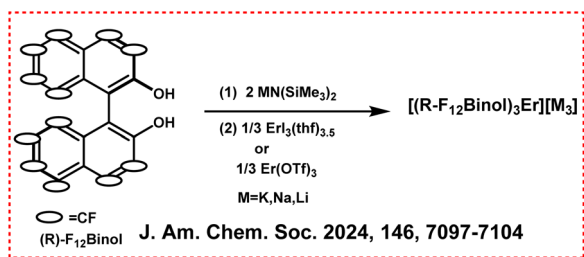
Scheme 40 Chemical structures of the ligands and Ln complexes [(R/S-F_{12} \text{Binol})_3\text{Er}][\text{M}]_3 . 90
