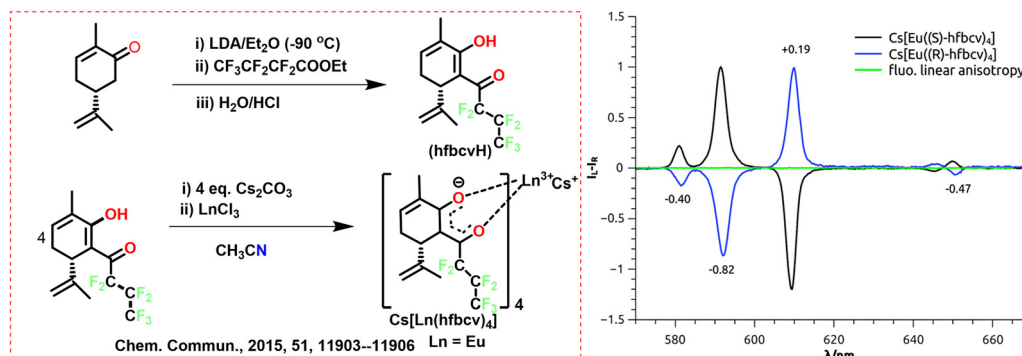
Scheme 10 (Left) Chemical structures of the ligands and Ln complexes ( R/S -Cs[Eu(hfbcv) _4 ]). 56 (Right) CPL spectra of Cs[Eu(( S )-hfbcv) _4 ] (black) and Cs[Eu(( R )-hfbcv) _4 ] (blue) on a quartz plate upon irradiation at 370 nm, with calculated g_{\text{lum}} values and fluorescence linear anisotropies (green). Reproduced from ref. 56 with permission from the Royal Society of Chemistry, copyright [2015]. 56
