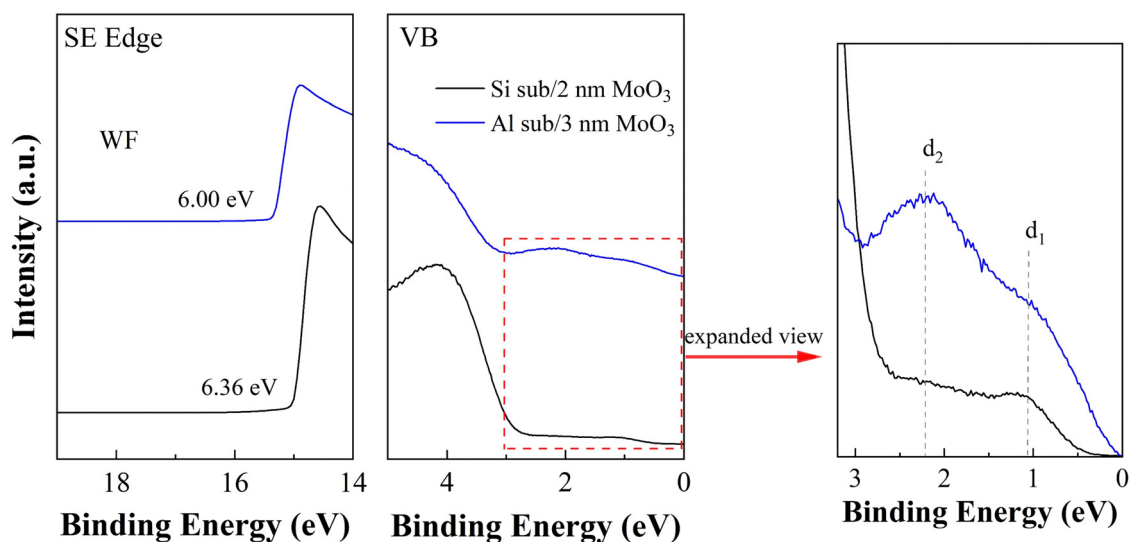
Fig. 5 The UPS spectra of the 2 nm \text{MoO}_3 film grown on Si substrate and 3 nm \text{MoO}_3 film grown on Al substrate. Gap states at various interfaces are labelled d_1 and d_2 .
