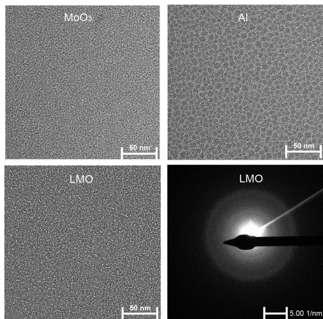
Fig. 4 Transmission electron microscopy (TEM) micrographs of 2 nm \text{MoO}_3 , 2 nm Al and the LMO films. TEM diffraction of the LMO is also shown.
