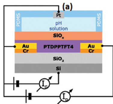
Fig. 37 (a) A pH sensor based on the BGBC dual-gate OFET and \text{SiO}_x as the active sensing layer (reproduced with permission from ref. 134. Copyright 2019, WILEY), (b) chemical structure of PTDPPTFT4 used as a semiconductor.
