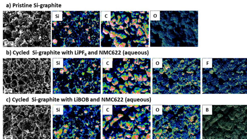
Fig. 4 SEM images and elemental mapping of the silicon-graphite composite (extracted from the cells containing NMC622(aqueous)): (a) pristine and after 280 cycles with (b) fluorinated and (c) fluorine-free electrolytes. The intensity of each element is color coded, ranging from black/blue for low intensity to pink/white for higher intensity.
