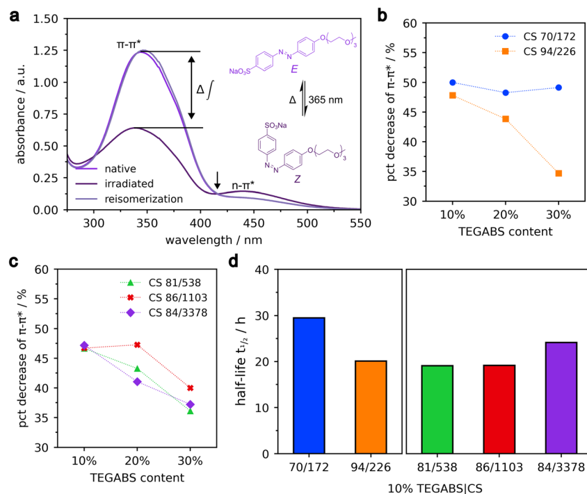
Fig. 7 UV-Vis characterization of native and irradiated TEGABS/CS thin films. In (a), the UV-Vis absorbance spectrum of the 10% TEGABS/CS 84/3378 film is depicted as native, irradiated ( \lambda_{exc} = 365 nm, dose of 3.3 J cm -2 ), and thermally reisolated states. The arrow represents the isosbestic point. The percentage decrease in area for the \pi-\pi^* transition from the native to isomerized state is shown for varying DDA (b) and DP (c), respectively. (d) Illustrates the influence of the DDA (left) and DP (right) on the thermal half-life of TEGABS at 30 °C.
