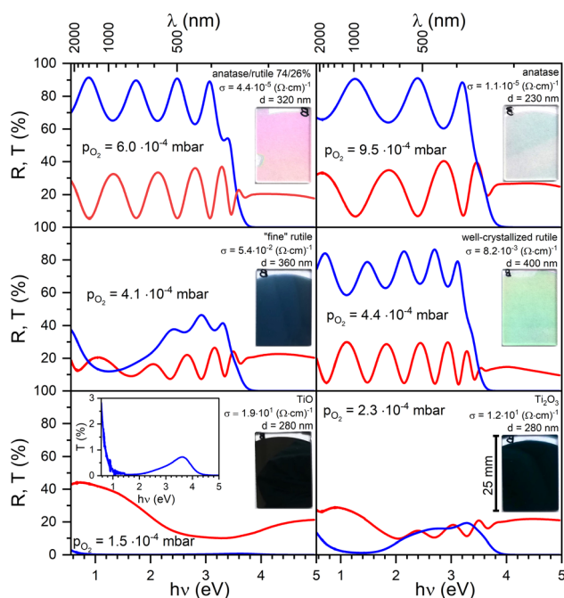
Fig. 2 Transmittance (blue) and specular reflectance (red) coefficients as a function of photon energy ( h\nu ) for titanium oxide thin films obtained at different oxygen partial pressures p_{O_2} ; conductivity at room temperature ( \sigma ) calculated from EIS measurements, thickness ( d ) and photographs of thin films deposited on amorphous silica substrates (dimensions 18 × 25 mm). In the inset: transmittance spectrum for TiO thin films.
