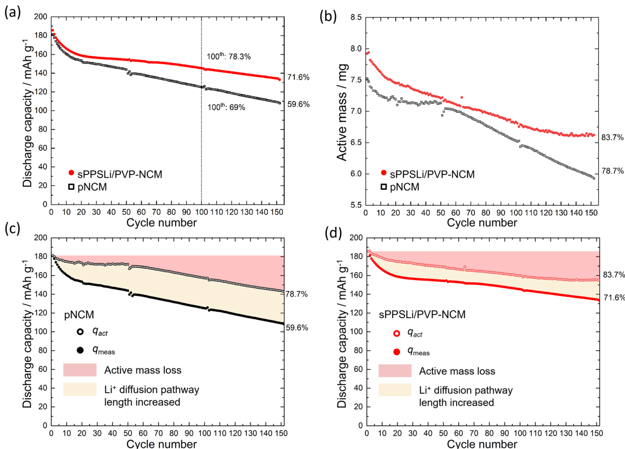
Fig. 4 (a) Cycling performance at 0.1C of \text{LiInSEB}^{\text{pNCM}} and \text{LiInSEB}^{\text{sPPSLi/PVP-NCM}} at 25 °C. (b) Corresponding evolution of m_{act} . For (c) pNCM and (d) sPPSLi/PVP-NCM, capacity loss is plotted, respectively, and split into the loss of m_{act} and the loss due to increased Li + diffusion pathway length. The pink area represents the loss of m_{act} . The yellow area illustrates the increasing Li + diffusion pathway length, determined as the difference between q_{meas} and q_{act} .
