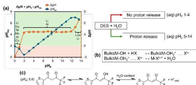
Fig. 1 (a) Effect of varying the initial pH of the aqueous phase on pH_{eq} and metal composition of the aqueous phase. (b) Reaction mechanism of metal oxides in acidic aqueous systems. 21 (c) Tautomerism of HTTA and its deprotonation form.
