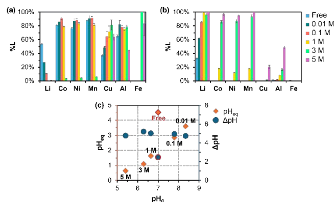
Fig. 2 Effect of varying the \text{H}_2\text{O}_2 concentration on the leaching efficiencies of the (a) organic phase and (b) aqueous phase. Leaching was conducted at 80 °C for 1 h with a solid-to-liquid ratio of 10 mg/mL and DES-to-aqueous phase volume ratio of 1:1. (c) Change in aqueous phase pH at equilibrium after leaching.
