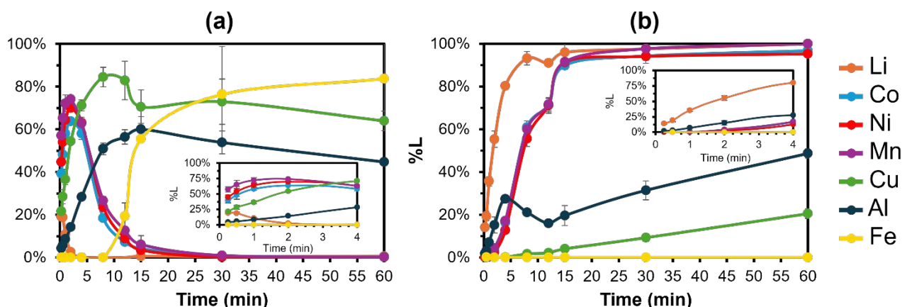
Fig. 3 Effect of varying the leaching duration on the leaching efficiencies of the (a) organic phase and (b) aqueous phase at 80 °C. Experiments were conducted using a solid-to-liquid ratio of 10 mg/mL, DES-to-aqueous phase volume ratio of 1:1, and 5 M \text{H}_2\text{O}_2 as the aqueous phase.
