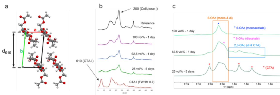
Fig. 6 Appearance of the CTA I (010) X-ray diffraction plane, in WAXS concomitant with CTA formation from comparison with NMR. (a) CTA I crystal structure with the (010) d-spacing highlighted. (b) Comparison of the experimental WAXS samples with a calculated diffraction pattern for CTA I (FWHM of 0.7). (c) Assigned acetate region in the diffusion-edited 1 H NMR spectra.
