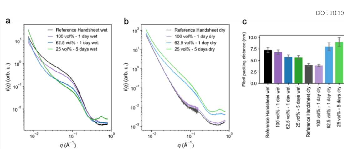
Fig. 4 SAXS results for the dry and hydrated (acetylated and reference) paper hand sheets. (a) SAXS intensities for the hydrated samples. (b) SAXS intensities for the dry samples. (c) Distance between elementary fibrils, as determined from the location of the peak maximum in the Kratky plots (ESI SFig. 8).
