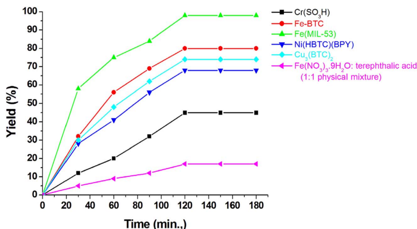
Fig. 4 Optimisation of different MOFs as catalysts for the synthesis of xanthenone (4a). a Reaction conditions: catalyst (20 wt%), benzaldehyde (0.71 mmol, 1.0 eq.), dimesityl dimedone (1.42 mmol, 2.0 eq.), ethanol (2.0 mL), reflux. Reaction monitored by HPLC.
