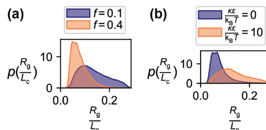
Fig. 5 Marginal distributions of the dimensionless radius of gyration, \frac{R_g}{L_c} , for SCNPs with (a) linker fraction f = \{0.1, 0.4\} and (b) backbone stiffness \frac{\kappa E}{k_B T} = \{0, 10\} .
