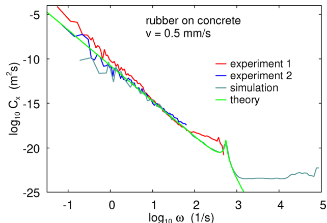
Fig. 12 The sliding distance power spectrum C_x(\omega) as a function of frequency. The experimental result is for rubber compound A sliding on a concrete surface, the theoretical result is for the reference case. Adapted from ref. 19.
