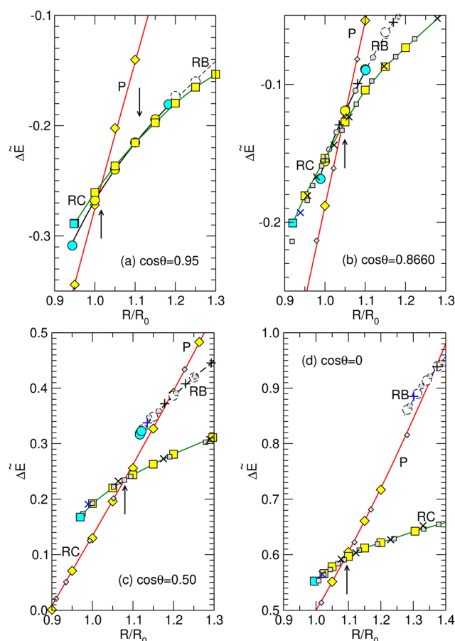
Fig. 14 Reduced surface free energies, \Delta \tilde{E} = \Delta E / (4\pi R_0^2 \gamma_{LG}) , for the P, RB, and RC states in Fig. 4, for wetting on a hollow-cylinder surfaces, for selected \theta values. The same legends used in Fig. 5 are followed here. The gray circles, gray squares, and gray diamonds are representative data for the P, RB, and RC states, read-off from Fig. 6 of ref. 28. Dashed lines and symbols represent unstable solutions, tested by the inflection condition (Appendix G) and by the off-center-of-mass numerical test (Section III C); they agree well with the gray dashed symbols from ref. 28, produced there by solving the Young–Laplace equation. The data from ref. 23 is plotted by plus and cross symbols. Plots (a)–(d) correspond to \cos \theta = 0.95, 0.886, 0.5, 0 , respectively.
