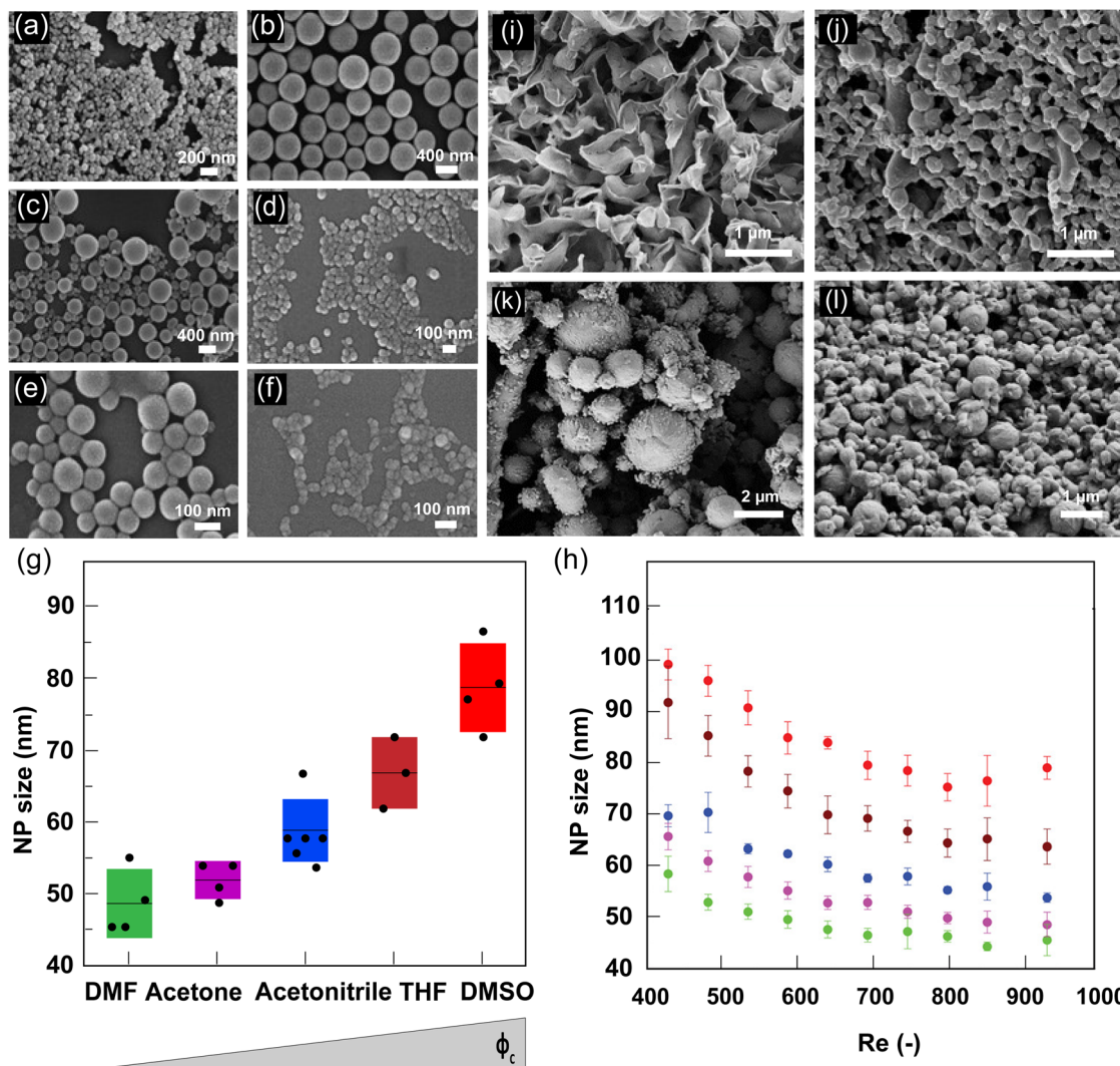
Fig. 3 Polymer nanoparticles (PNPs) prepared by nanoprecipitation. (a)–(f) SEM image of the PNPs prepared using two polymer poly(MMA-stat-pyMAA) (PMMA) and copolymer poly(MMA-stat-EA). (a)–(c) PMMA; (d)–(f) PMMA and copolymer. The mixing conditions are by dripping acetone to water (a) and (d), by dialysis of N,N -dimethylacetamide (c) and (f), or by dripping water to acetone (b) and (e). 49 Variation of the PNP size as a function of (a) solvents under constant mixing kinetics ( Re = 749 ), and (b) Reynolds number ( Re = 400 – 1000 ). 45 (i)–(l) Field emission scanning electron microscopic image representing the variation of PNP size on the final polymer concentrations (i) 0 \text{ mg mL}^{-1} , (j) 1 \text{ mg mL}^{-1} , (k) 2 \text{ mg mL}^{-1} , and (l) 5 \text{ mg mL}^{-1} from an initial polymer concentration of 5 \text{ mg mL}^{-1} . 53
