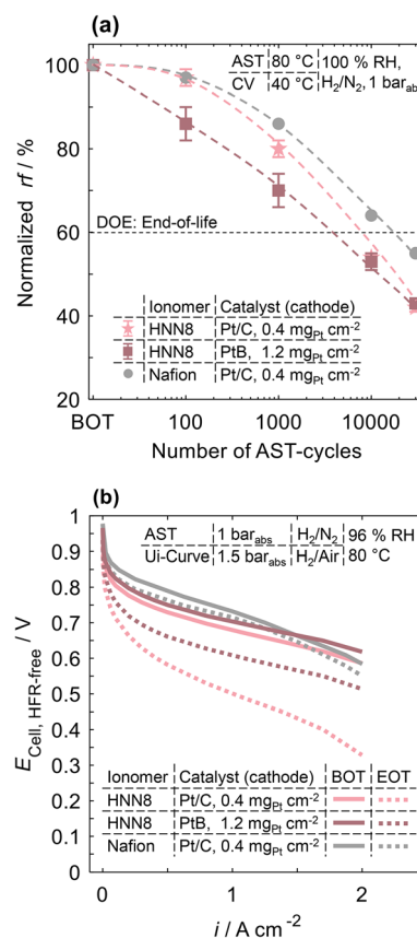
Fig. 6 (a) Normalized cathode roughness factor rf ( rf/rf^{BOT} ) as a function of AST-cycles, and (b) polarization curves at BOT and EOT of fully HC- and fully PFSA-based CCMs with varying cathode electrocatalyst. The cathodes utilize Nafion D2020 (I/C = 0.8, 50 wt% Pt/C, Pt loading of 0.41 ± 0.01 mg Pt cm -2 ) and Pemion® HNN8 with (i) 50 wt% Pt on high surface area carbon (Pt/C, 0.42 ± 0.02 mg Pt cm -2 ), and (ii) unsupported Pt (PtB, 1.2 ± 0.01 mg Pt cm -2 ).
