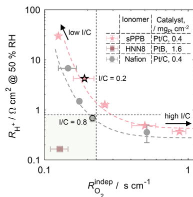
Fig. 5 Protonic resistance R_{H^+} (measured at 50% RH) versus pressure-independent O 2 transport resistance R_{O_2}^{indep} (measured at 80% RH) for cathode CLs utilizing 50 wt% Pt/C (Pt loading of 0.4 mg Pt cm -2 ) and different contents of sPPB or Nafion D2020 (extracted from Fig. 2a and b, with black framed data points refer to the “standard” I/C ratio of operation). The square marked data point refers to a cathode CL utilizing 2.5 wt% Pemion® with unsupported Pt (PtB) loading of 1.6 mg Pt cm -2 . All data points were measured at 80 °C.
