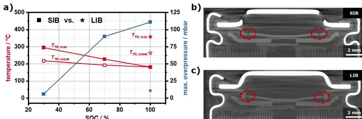
Fig. 3 (a) Summary of the SOC-dependent TR-behaviour, by means of T_{\text{TR,onset}} , T_{\text{TR,max}} and p_{\text{max}} of the SIB- and LIB-cells investigated. The T_{\text{TR,max}} -values of the SIB-cells at 70% SOC and 100% SOC are not reasonable due to the strong jelly roll ejection at these SOC. CT-images of the top of (b) the SIB-cell and (c) the LIB-cell.
