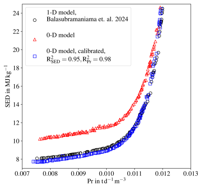
Fig. 2 Comparison of calculated specific energy demand (SED) and productivity (Pr) for various steam-assisted cycle designs using APDES sorbent, between 1-D model, 0-D model, and calibrated 0-D model.
