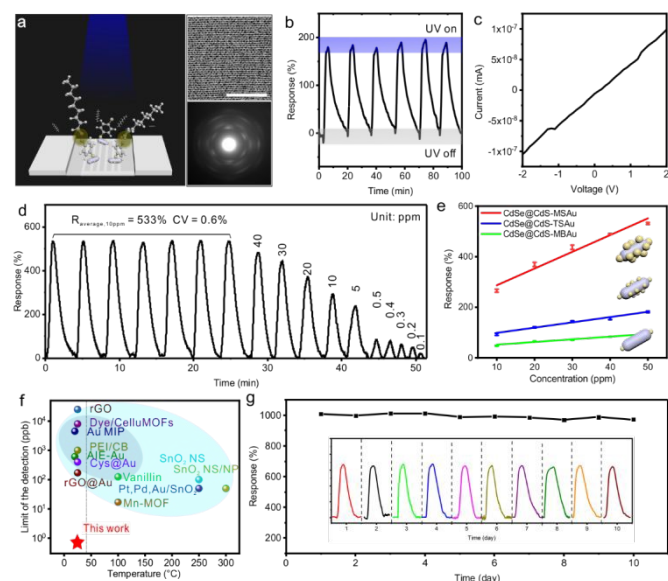
Figure 3. Detection performance of trans-2-nonenal. (a) Schematic diagram of the sensor with the modified sensing materials with 4-bromobenzenethiol and interdigital electrodes for trans-2-nonenal. Typical TEM image of CdSe@CdS-MBAu assembly at the top right and small angle electron diffraction at the bottom right. Scale bar, 100 nm. (b) Response curve of the sensor under UV irradiation. (c) Volt-ampere characteristic curve. (d) Concentration-dependent response-recovery curves. (e) Response-concentration plots of CdSe@CdS, CdSe@CdS-TSAu, CdSe@CdS-MSAu and CdSe@CdS-MBAu sensors. (f) Comparison of limits of detection for trans-2-nonenal, homologous compounds and C9 alkanals in optical sensors (dark blue shadow) and chemoresistive sensors (light blue shadow). According to IEC 60601-1-11 standard for medical electrical equipment in home healthcare environments,
