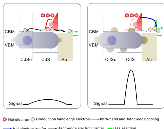
Scheme 1. Schematic diagram of chemical physical processes for gas-sensing reactivity in CdSe@CdS-Au with two-tips Au domains and CdSe@CdS-Au with large multi-site Au domains, as well as the corresponding detection signal variations. The term response signal refers to the resistance value.
