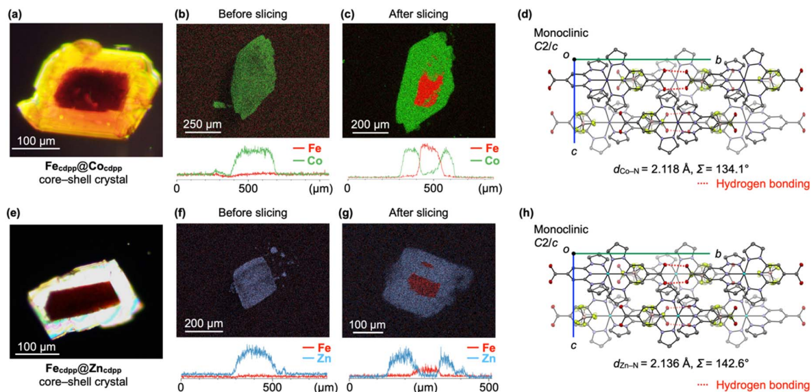
Fig. 3 (a) POM image of \text{FeCdpp@CoCdpp} . (b and c) SEM-EDX elemental maps (top) and total area traces (bottom) of \text{FeCdpp@CoCdpp} (b) before and (c) after slicing by a ultramicrotome. (d) Crystal structure of \text{CoCdpp} in the outer shell along the a -axis. (e) POM image of \text{FeCdpp@ZnCdpp} . (f and g) SEM-EDX elemental maps (top) and total area traces (bottom) of \text{FeCdpp@ZnCdpp} (f) before and (g) after slicing by a ultramicrotome. (h) Crystal structure of \text{ZnCdpp} in the outer shell along the a -axis.
